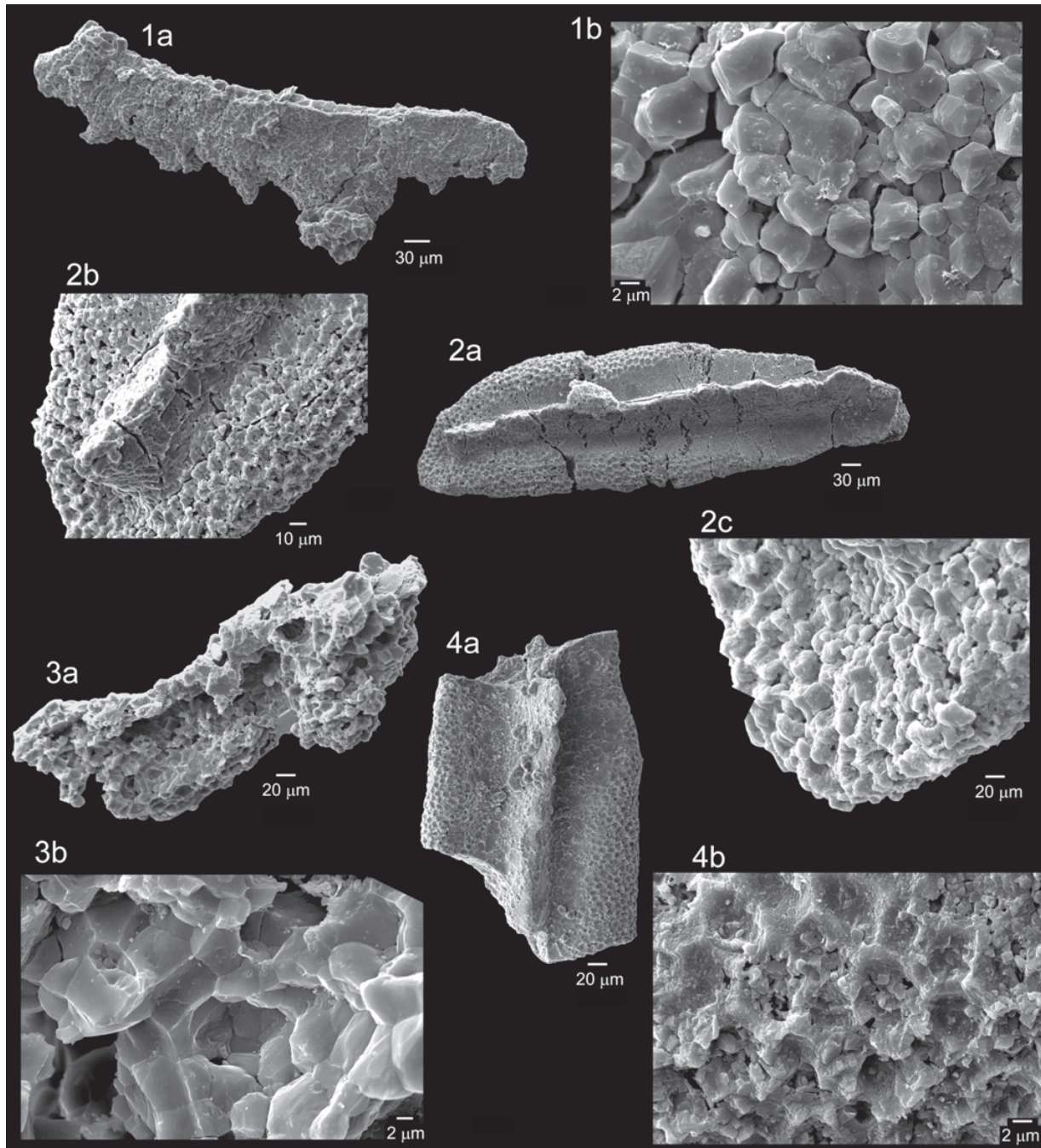
Fig. 11. Metamorphosed and only slightly ductile deformed conodonts from the Late Anisian or Late Ladinian to ?Early Carnian of locality Županje 2 with Conodont Colour Alteration (CAI) values of CAI 5.5–6.0. Samples SRB 111 and SRB 112. 1a — Neogondolella cf. cornuta . CAI 5.5–6.0. 1b — Enlarged part from 1a showing the strong recrystallization and growth of the apatite crystals. The typical surface is completely destroyed by recrystallization. 2a — Neogondolella cf. eotrammeri . CAI 5.5–6.0. 2b — Enlarged platform end of the specimen figured in 2a showing the complete recrystallization of the ornamentation. 2c — Growth of apatite crystals, enlarged part from 2b. 3a — Gondolella cf. excelsa , extremely recrystallized. 3b — Same specimen, enlarged part showing the strong recrystallization and growth of the apatite crystals. 4a — Broken piece from the platform element of Neogondolella cf. inclinata . 4b — Enlarged part from 4a showing strong recrystallization and growth of apatite crystals in the area of platform ornamentation.
