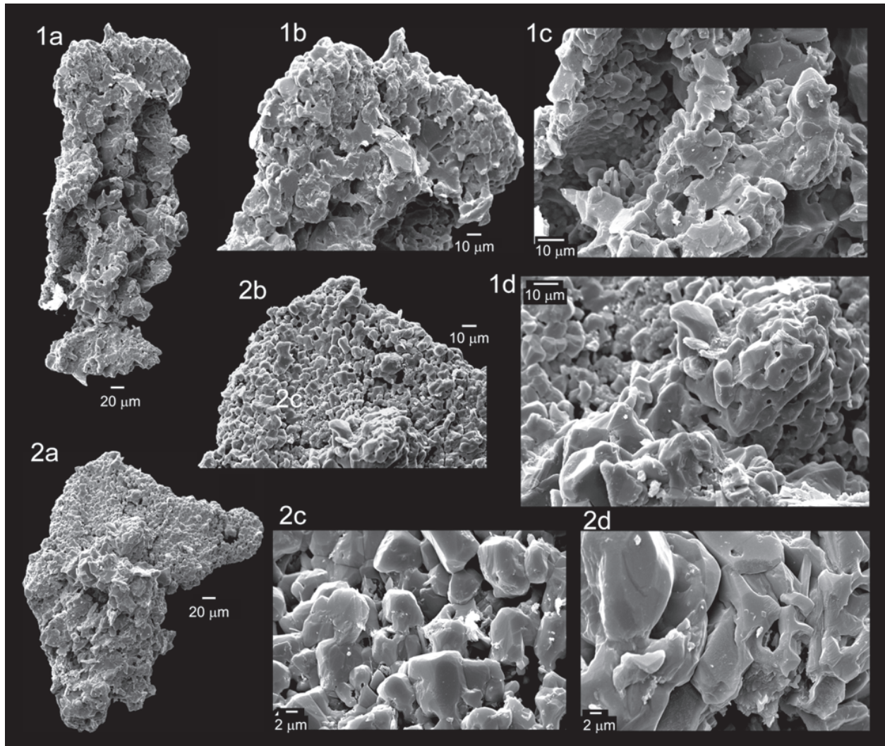
Fig. 10. Metamorphosed and ductilely deformed conodonts ( Metapolygnathus polygnathiformis ) with Conodont Colour Alteration (CAI) values in average CAI 5.5–6.0 from Kopaonik, Brzeće section (sample SRB 115). These conodonts come from probably Upper Carnian grey metalimestones. 1a — Strongly recrystallized and corroded specimen. CAI 5.5–6.0. 1b — Platform end enlarged showing strong recrystallization and growth of the apatite crystals. 1c — Enlarged detail with strong recrystallization and partial corrosion of the surface. 1d — Detail of the surface with relatively large apatite crystals. 2a — Strongly recrystallized and slightly deformed specimen. CAI 6.0. 2b — Platform end enlarged showing strong recrystallization and growth of the apatite crystals. The original surface is completely destroyed by recrystallization. 2c — Enlarged detail showing strong recrystallization and growth of individual apatite crystals. 2d — Enlarged detail showing strong recrystallization of apatite and enlargement of the crystallites.
