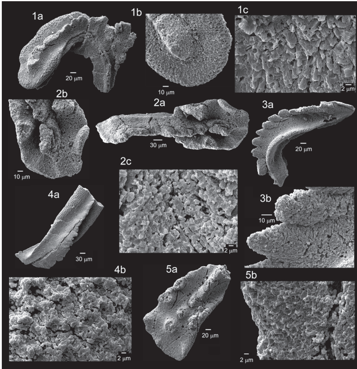
Fig. 8. Metamorphosed and deformed conodonts with Conodont Colour Alteration (CAI) values 5.5–6.0 from the Studenica section (Sample SRB150). These conodonts occur in grey cherty metalimestones and are of Early Norian (Laciian) age. 1a — Ductilely deformed Norigondolella navicula . In this view the original ornamentation on the platform surface looks undeformed. 1b — Platform end of Norigondolella navicula , enlarged, showing complete recrystallization of the original ornamentation by apatite crystal growth. 1c — Enlarged detail of 1b showing the growth of the apatite crystals. Corrosion is missing. 2a — Slightly deformed Epigondolella triangularis . 2b — Enlarged platform end showing the complete and relatively homogeneous recrystallization of the conodont. 2c — Enlarged detail showing the growth of apatite crystals. 3a — Ductilely deformed Norigondolella navicula . 3b — Recrystallized fabric, enlarged from 3a. 4a — Deformed and recrystallized part of ? Norigondolella navicula . The original ornamentation on the platform surface is preserved and looks undeformed. 4b — Enlarged view on the ornamentation showing complete recrystallization of the ornamentation. 5a — Undeformed but totally recrystallized Epigondolella triangularis . 5b — Recrystallized fabric, enlarged from 5a.
