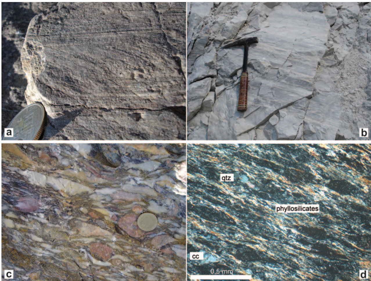
Fig. 5. Lower and Middle Triassic lithofacies. a — Cross-bedded sandstone, Lower Werfen Formation, Kopaonik area (7486570/4795890). b — Calcite-mylonite attributed to the Steinalm Formation (Anisian), Studenica quarry. c — Polymictic breccia overlying the Steinalm Formation, Studenica quarry. d — Tuffite, presumably Anisian/Ladinian boundary, Studenica quarry, thin-section crossed polarizers.
