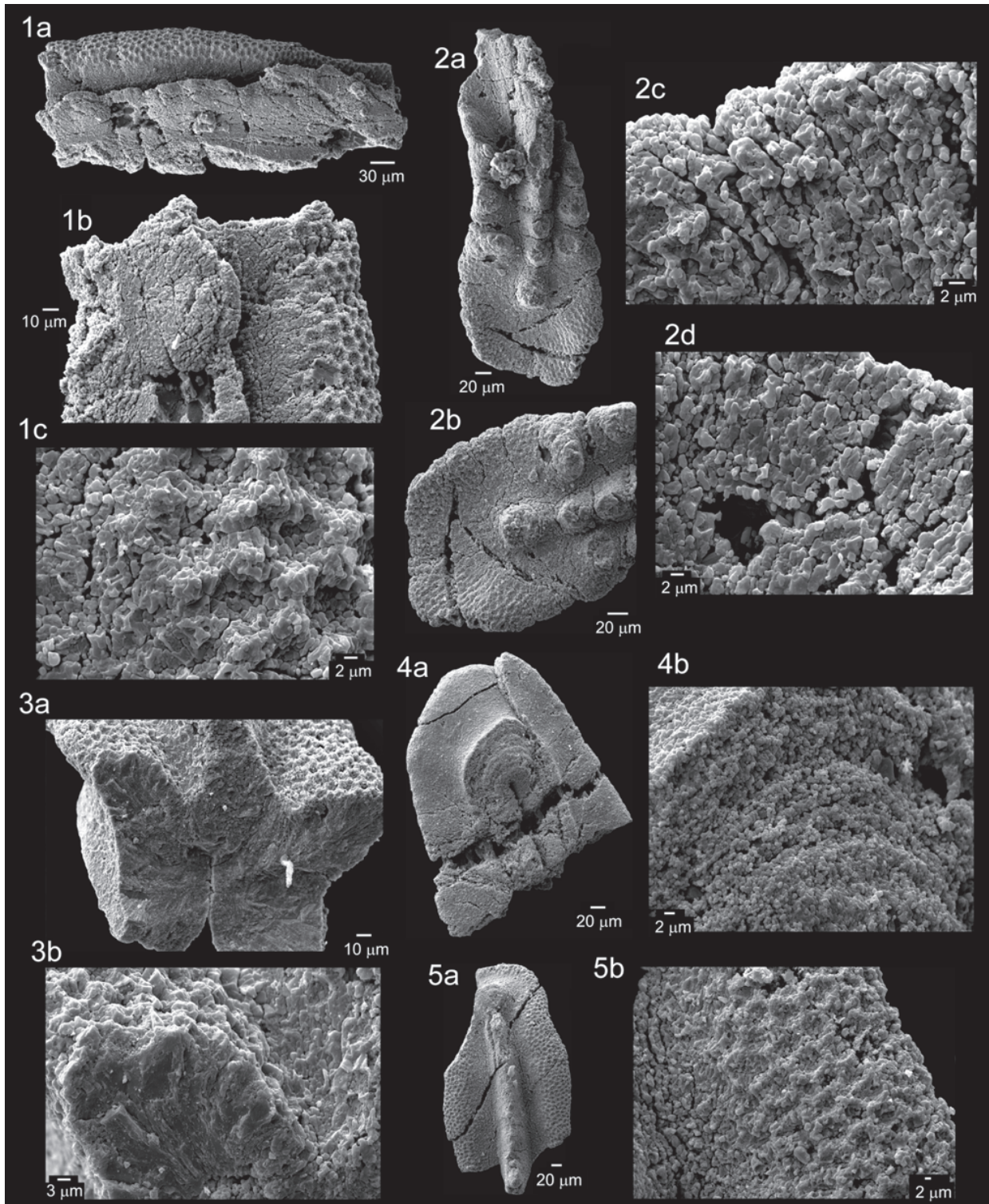
Fig. 9. Metamorphosed and partly ductilely deformed conodonts with Conodont Colour Alteration (CAI) values 5.5–6.0 from the Studenica section (sample SRB 153). These conodonts are from Lower Norian (Lacian) grey cherty metalimestones. 1a — Slightly deformed and recrystallized Norigondolella sp. From this view, the original ornamentation on the platform surface looks undeformed. 1b — Platform end, enlarged, showing complete recrystallization. 1c — Enlarged view on the ornamentation showing the complete recrystallization of the ornamentation. 2a — Undeformed but totally recrystallized Epigondolella sp. 2b — Enlarged view of platform showing strong recrystallization. 2c, d — Details of recrystallization, enlarged from 2b. 3a — Broken Norigondolella sp. showing recrystallization in the inner part of the conodont. 3b — Enlarged detail from 3a. 4a — Basal view of Norigondolella navicula . 4b — Enlarged detail from 4a. 5a — Broken Norigondolella cf. hallstattensis . The original ornamentation on the platform surface is preserved and looks undeformed. 5b — Enlarged view of the ornamentation showing complete recrystallization of the ornamentation.
