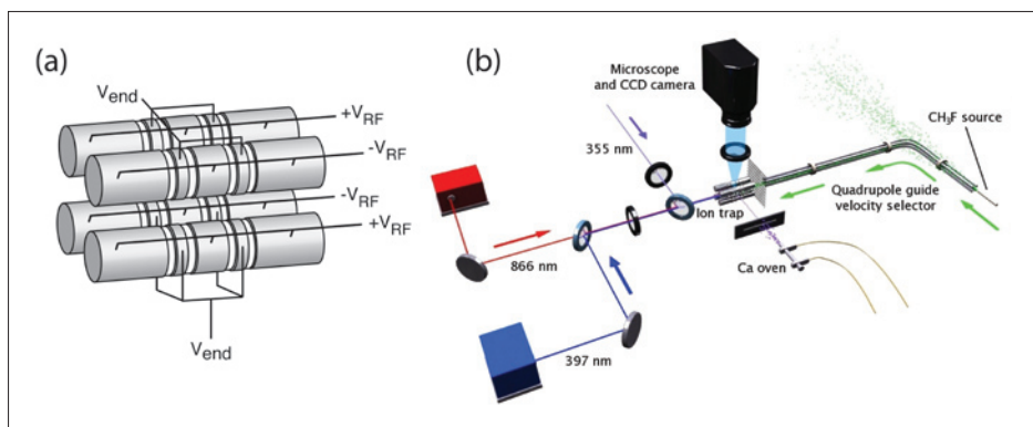
Fig. 1. (a) Schematic representation of a linear Paul trap. (b) Experimental setup to study ion-molecule reactions at very low translational temperatures ( T_{\text{trans}} \geq 1 K). Left-hand side: linear Paul trap used for the laser and sympathetic cooling of ions with cooling lasers and imaging system. Right-hand side: quadrupole-guide velocity selector to generate continuous beams of translationally cold polar neutral molecules. See text for details. Reproduced from ref. [10].
