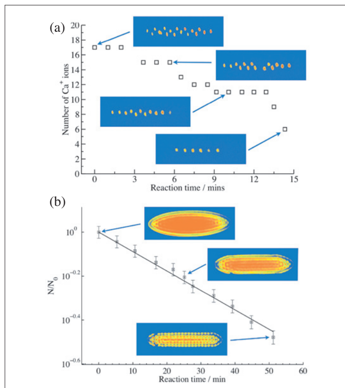
Fig. 4. Decrease of the number of laser-cooled \text{Ca}^+ ions as a function of the reaction time with velocity-selected \text{CH}_3\text{F} molecules for (a) a small Coulomb crystal of 17 ions and (b) a large Coulomb crystal of \approx 250 ions. The solid line in (b) represents a fit of the data to a pseudo-first order rate law from which the bimolecular rate constant k_{\text{bi}} of the reaction can be determined. Reproduced from ref. [11].
