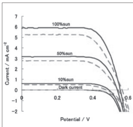
Fig. 4. Current-voltage curves for DSCs prepared using [\text{Cu}(1)_2]^+ (broken curves) and [\text{Cu}(2)_2]^+ (solid curves). [9]
