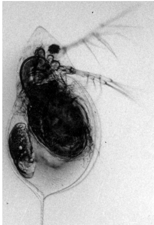
Figure 2.4 Daphnia cucullata . Adult female with one embryo in her brood chamber. This female comes from a laboratory culture of a clone originally isolated from Klostersee in southern Bavaria, Germany.
