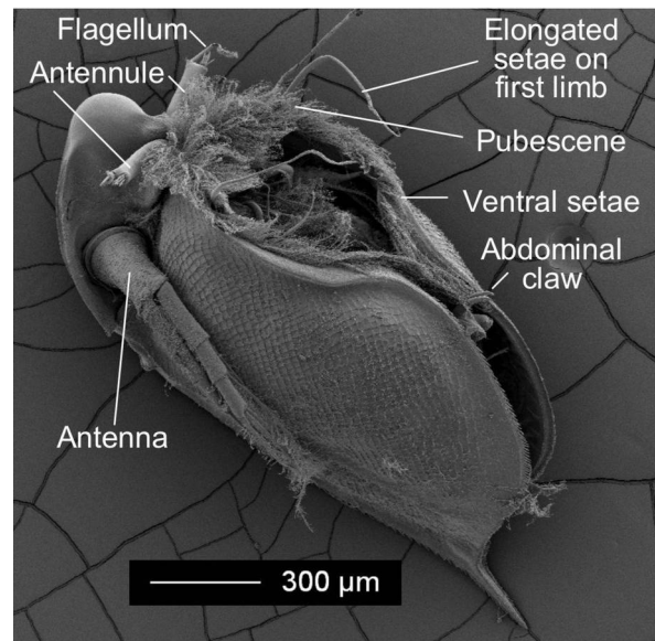
Figure 2.16 Scanning electron microscopic of an adult male Daphnia magna . A male D. magna from a laboratory population of a clone isolated from a rock pool in southern Finland. Photo by Frida Ben-Ami, Basel University.
