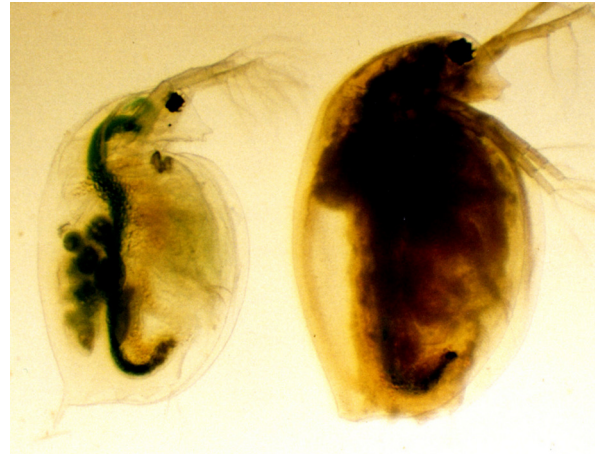
Figure 3.1 D. magna with (right) and without (left) P. ramosa infection. The parasite can be seen as a dark cloudy mass filling the entire body. The brood pouch of the infected female is empty, whereas the healthy female carries a clutch of eggs. This photograph was taken with the light shining from below. The infected host is larger than the healthy female, which is typical for P. ramosa infections.
