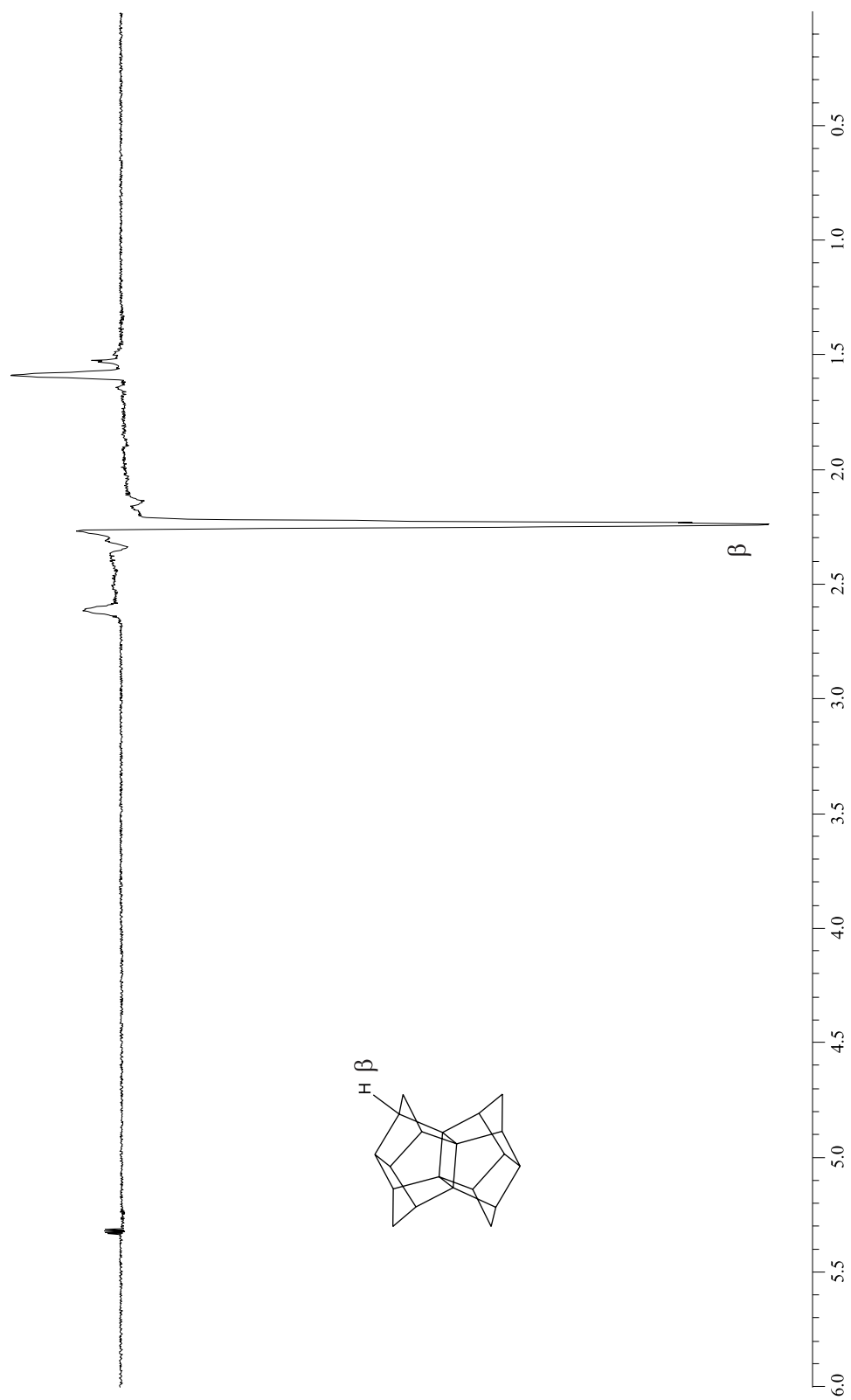
Figure 4.4: ^1\text{H} -CIDNP spectrum of [1.1.1]pagodane P1
