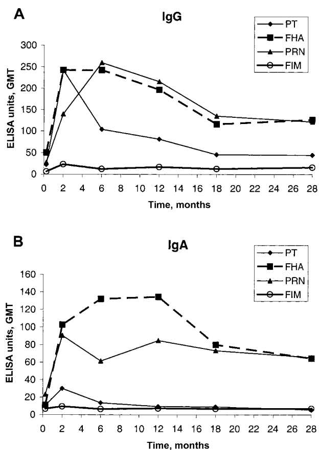
Figure 1. Geometric mean titers (GMTs), as determined by ELISA, of antibodies to pertussis toxin (PT), filamentous hemagglutinin (FHA), pertactin (PRN), and fimbriae type 2 and type 3 (FIM) in serum samples obtained at selected times after the onset of illness in 11 adults with pertussis. A , IgG antibody; B , IgA antibody.
