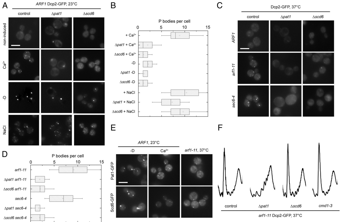
Figure 6. Pat1 and Scd6 are required for PB assembly in secretory transport mutants and upon Ca 2+ treatment. (A) PBs were induced in wild type, \Delta pat1 or \Delta scd6 mutant cells expressing Dcp2-GFP by treatment with 200 mM CaCl 2 or 0.5 M NaCl, or after incubation in rich medium lacking a carbon source (-D) for 15 min at 23°C. Although PB induction by osmotic stress or starvation was not affected in the deletion mutants, a strong reduction of PB number was observed after Ca 2+ treatment. (B) Quantification of PBs in the \Delta pat1 or \Delta scd6 strains compared with wild-type. See Figure 1B for details on the representation. (C) Pat1 and Scd6 are required for assembly of multiple PBs in secretion mutants. Wild type, arf1-11 , and sec6-4 expressing Dcp2-GFP and deleted for either PAT1 or SCD6 were shifted to 37°C for 1 h. Deletion of PAT1 or SCD6 abolished the multiple PB phenotype in secretion mutants. (D) Quantification of PBs in secretory mutants deleted for PAT1 or SCD6 after a shift to the nonpermissive temperature. See Figure 1B for details on the representation. (E) PBs were induced in wild-type or arf1-11 cells expressing either Pat1-GFP or Scd6-GFP by incubation in rich medium lacking a carbon source (-D), treatment with 200 mM CaCl 2 for 15 min at 23°C, or a shift to 37°C for 1 h, respectively. Both Pat1-GFP and Scd6-GFP behaved similarly to Dcp2-GFP and were found in multiple PBs after Ca 2+ treatment or in the secretory mutant after shift to the nonpermissive temperature. (F) arf1-11 cells deleted for PAT1 or SCD6 , or carrying the cmd1-3 allele were shifted to 37°C for 1 h and their polysome profile recorded. Although all three strains do not induce multiple PBs under this condition, translation is derepressed only in the strain deleted for PAT1 . Scale bars, (A, C, and E) 5 \mu m.
