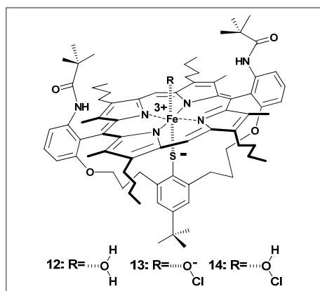
Fig. 2. Enzyme mimics of chloroperoxidase (CPO).
