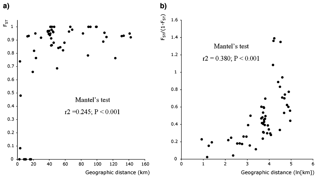
Figure 3. IBD observed between French Vipera ursinii ursinii populations using (a) the divergence between the mitochondrial cytochrome b (1116 bp; Mantel test: r^2 = 0.245 ; P < 0.001 ) and (b) 6 microsatellite markers (Mantel test: r^2 = 0.380 ; P < 0.001 ). We used the uncorrected distance for the mitochondrial analysis due to some F_{ST} = 1 (with the correction F_{ST}/[1 - F_{ST}] = \infty ).
