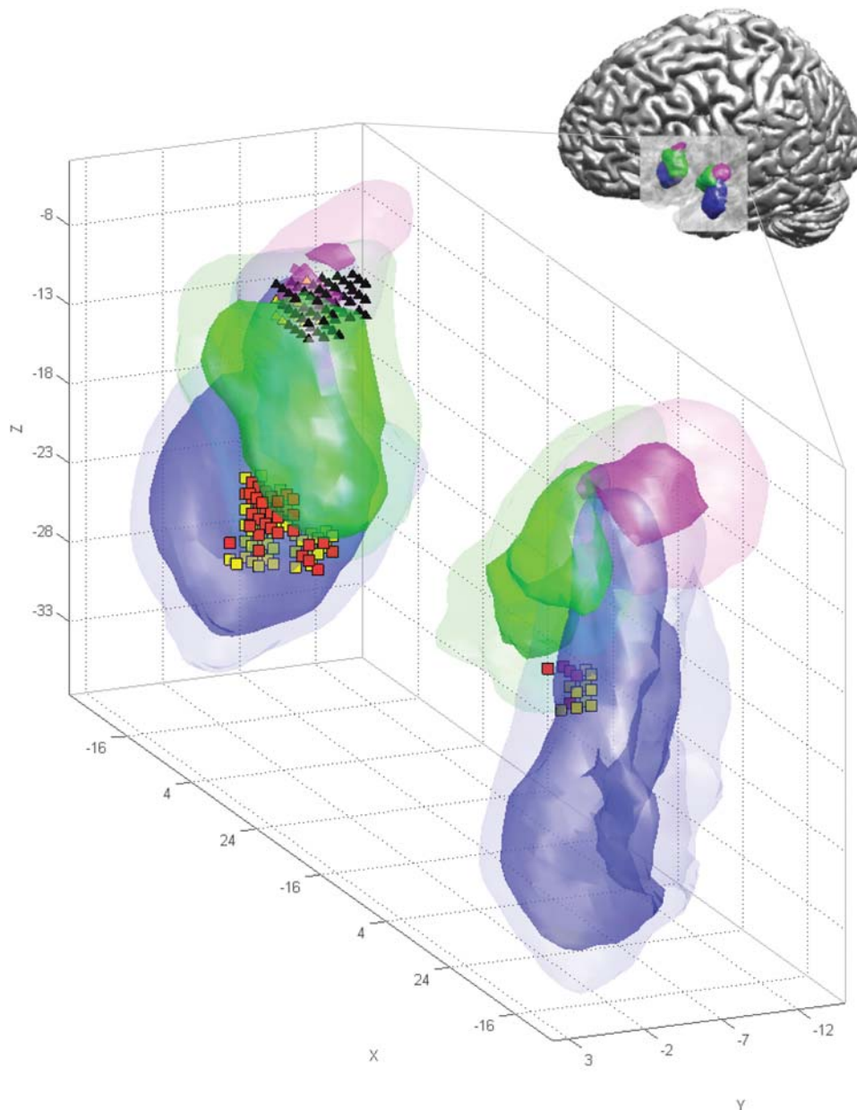
Figure 4. Human amygdala responses to music in probabilistically defined anatomical regions. The volumes with at least 50% and 80% probability to belong to the three major amygdala subregions: LB=laterobasal group (blue), SF=superficial group (green), and CM=centromedial group (magenta) are rendered with high (for 50% probability) and low (for 80% probability) transparency. Voxels with a significant increase in BOLD signal to music presentation are displayed as red or yellow squares ( p < 0.05 , corrected for multiple comparisons, see material and methods for further details). Voxels with a significant signal decrease are displayed as black or yellow triangles. Anatomical probabilities for red and black responses were 50% to 60%, for yellow responses 70% or above. The majority of significant effects was found in the left amygdala. Positive effects were found in both right and left LB and SF (c.f. Tab. 2), negative effects were localized in left LB, SF and CM. For visualization, probability maps were smoothed using a spatial filter with a 5 mm isometric Gaussian convolution kernel. doi:10.1371/journal.pone.0000307.g004
