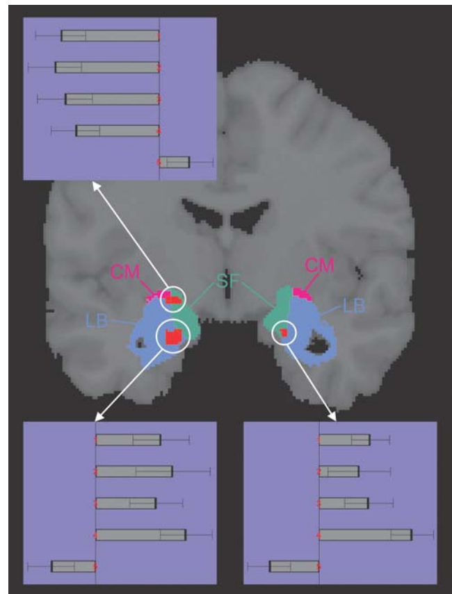
Figure 3. Music-related amygdala responses. The extent of the amygdala subregions LB, SF, and CM defined by maximum-probability maps (MPMs, [28]) are rendered in blue, green, and magenta, respectively, on a coronar section. Regions with significant ( p < 0.05 , corrected for multiple comparisons in the search volume) music-related responses are shown in red. The BOLD percentage signal change (PSC) of each of the three activation sites in the four music conditions (1: dissonant slow, 2: consonant slow, 3: dissonant fast, 4: consonant fast) is presented as mean and standard error. The fifth PSC value refers to the time period during which subjects evaluated the emotional effect evoked by the preceding musical piece, compared with rest. In the left amygdala, a cluster with positive responses to all music conditions was mainly located in LB and a cluster with negative responses was mainly found in SF and CM (see also Tab. 2). A smaller cluster with consistently positive responses was also found in the right amygdala approximately in the mirror position to the positively responding left cluster. doi:10.1371/journal.pone.0000307.g003
