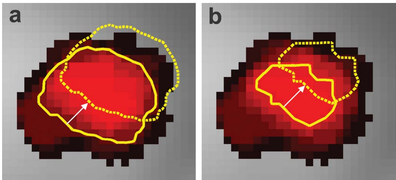
Figure 2. Simulated effect of probabilistic region of interest (ROI) definition on robustness against localization errors. In (a) and (b), axial sections through the laterobasal part (LB) of the left amygdala are shown at z = -29 (MNI coordinate system). Probabilities to belong to LB are color coded with black = 10% and pure red = 100%. In (a), the probabilistic ROI is defined as the area with \geq 50\% probability to belong to LB (solid yellow line). As a consequence of a simulated localization error which consists of a linear shift of approximately 4 mm (indicated by the white arrow) the true measured volume is localized as indicated by the dashed yellow line, containing voxels with little or no probability to belong to LB. In contrast, when restricting the ROI to voxels with 90% or 100% LB probability (b) and given an equally large localization error, the true measured volume is still entirely located within the area of LB. In this way, the robustness against localization errors could be increased, counteracting potential localization errors while still maintaining excellent anatomical specificity. doi:10.1371/journal.pone.0000307.g002
