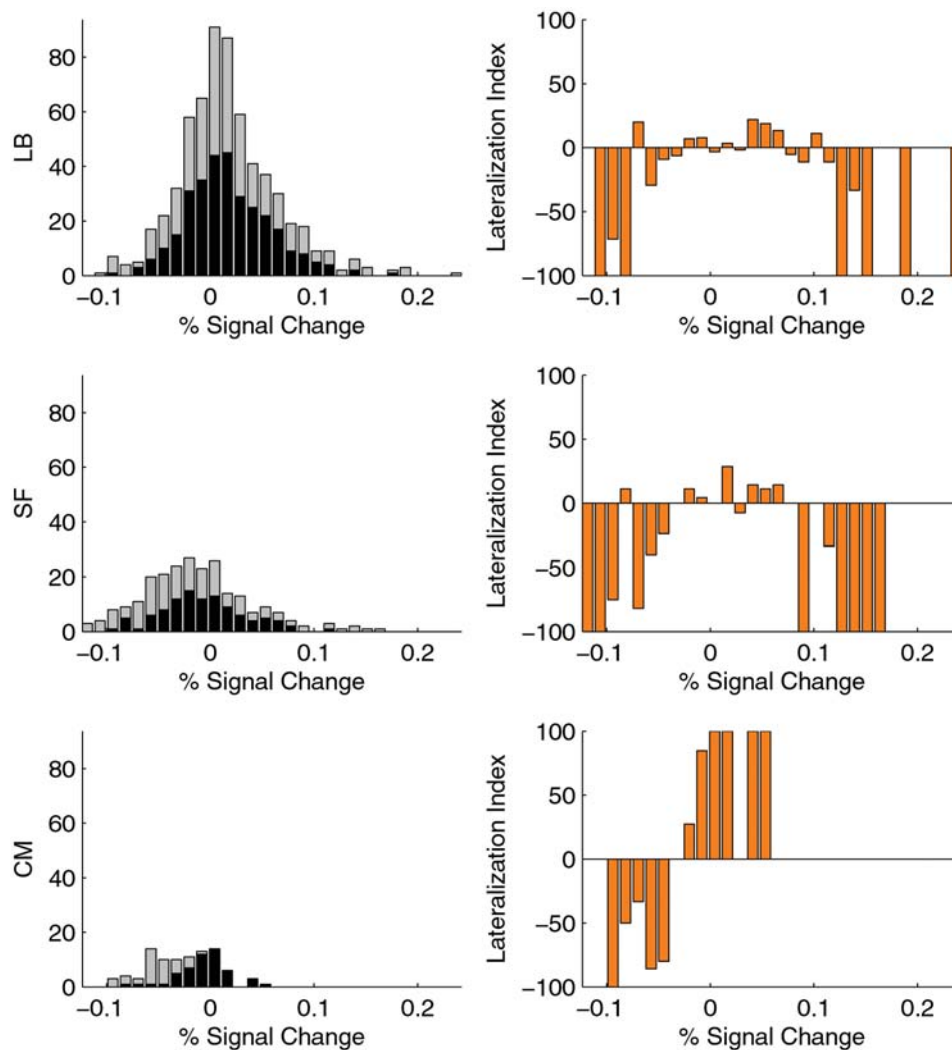
Figure 5. Lateralization patterns in the major subdivisions of the human amygdala. Histograms on the left show the distribution of BOLD percentage signal change (PSC) for voxels in: LB = laterobasal group, SF = superficial group, and CM = centromedial group. Values for the right (black) and left (light grey) amygdala are shown in a stacked way. For each PSC bin, a lateralization index (LI) was calculated. LIs of 100, -100, and 0 indicate purely right-sided, purely left-sided, and symmetrically distributed effects, respectively. LB and SF showed a similar lateralization pattern of both extremely positive and negative PSC predominating in the left amygdala. CM showed a different lateralization pattern with negative PSC predominating in the left and positive PSC in the right amygdala. doi:10.1371/journal.pone.0000307.g005
