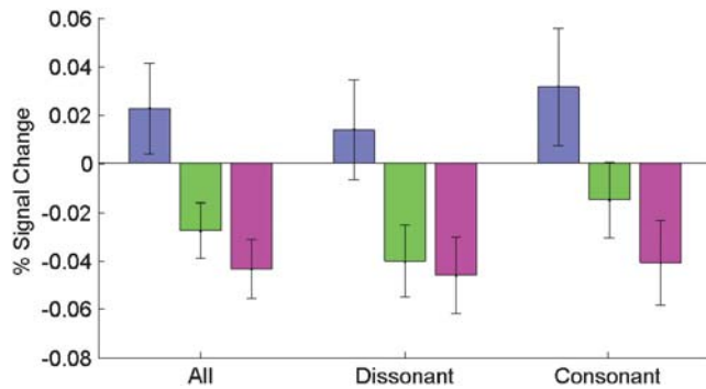
Figure 6. Response differences between amygdala subregions. We performed a region of interest (ROI) analysis to statistically evaluate response differences between the core regions (with 90–100% assignment probability) of the three amygdala subregions (see Material and Methods for further details). Bars in the above figure show the result of three averaging steps: first across all voxels of a given area, then either across all four music conditions, the dissonant conditions, or the consonant conditions, and finally across the 14 subjects. Results are given for left LB, SF, and CM in blue, green, and magenta. Error bars indicate the standard error of the mean from of the average across subjects. In each case, the differences between left LB and left SF and CM were significant at p < 0.005 . There were no corresponding significant differences in the right amygdala. doi:10.1371/journal.pone.0000307.g006
