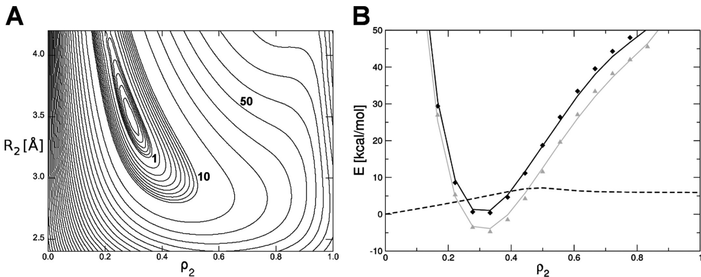
FIGURE 2. A, contour plot of the potential energy surface resulting from the DFT scan on model C along \rho_2 = (r_2 - 0.8)/(R_2 - 1.6) and R_2 . B, example of the fitting process used to avoid double counting of the molecular mechanics nonbonded terms. V_{PT} is fitted to the difference between the DFT energy and V_{MM} . The slice shown is for constant R_2 = 3.36 Å. Black diamonds, V^{ef}(\vec{x}) , which is DFT energy; dotted black line, V_{MM}(\vec{y}) , which is the MM energy calculated when V_{PT} is set to 0; gray triangles, V^{ef}(\vec{x}) - V_{MM}(\vec{y}) ; gray line, V_{PT}(R_2, \rho_2, \theta_2) , obtained from a least-squares fit of the asymmetric double minimum potential shown in the supplemental data to the gray triangles; black line, total fitted MMPT potential V^{fit}(\vec{x}) .
