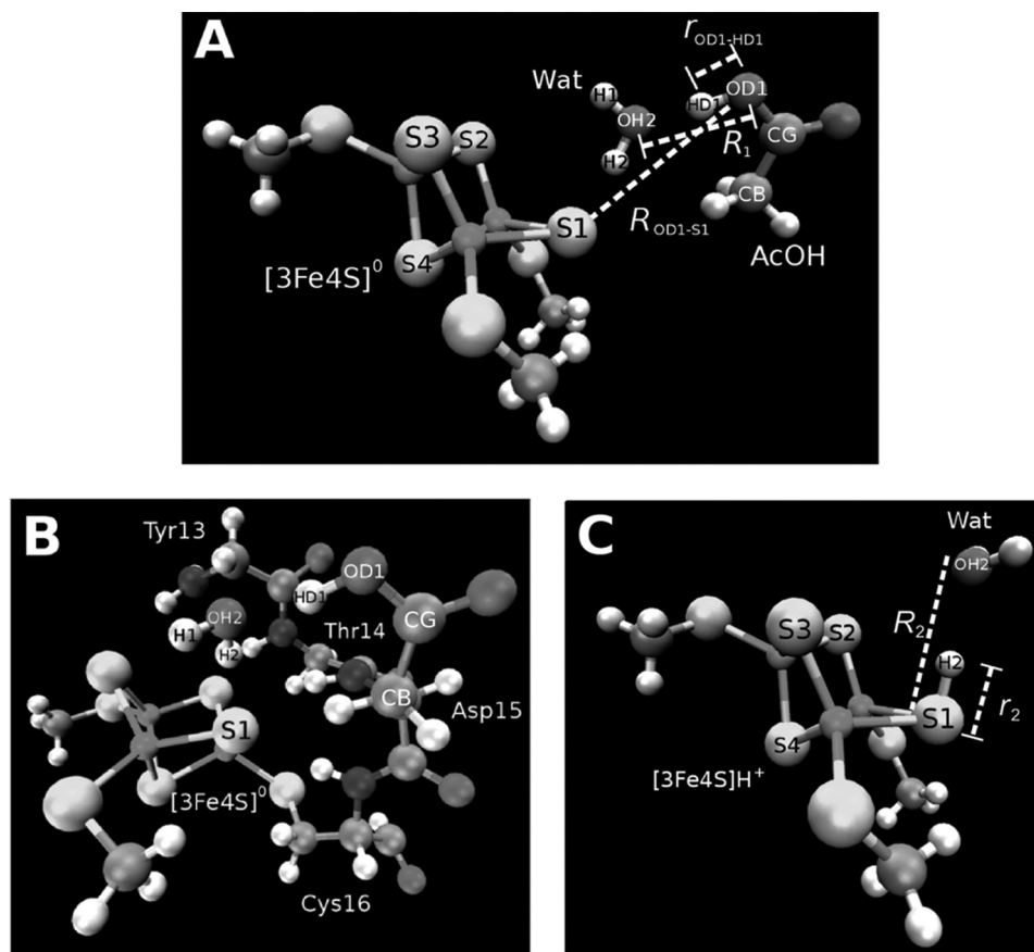
FIGURE 1. A , small model system used in the DFT energy scan. B , large model system for the DFT energy scan. C , model system used to calculate the two-dimensional PES used for fitting MMPT function. Wat , water.
