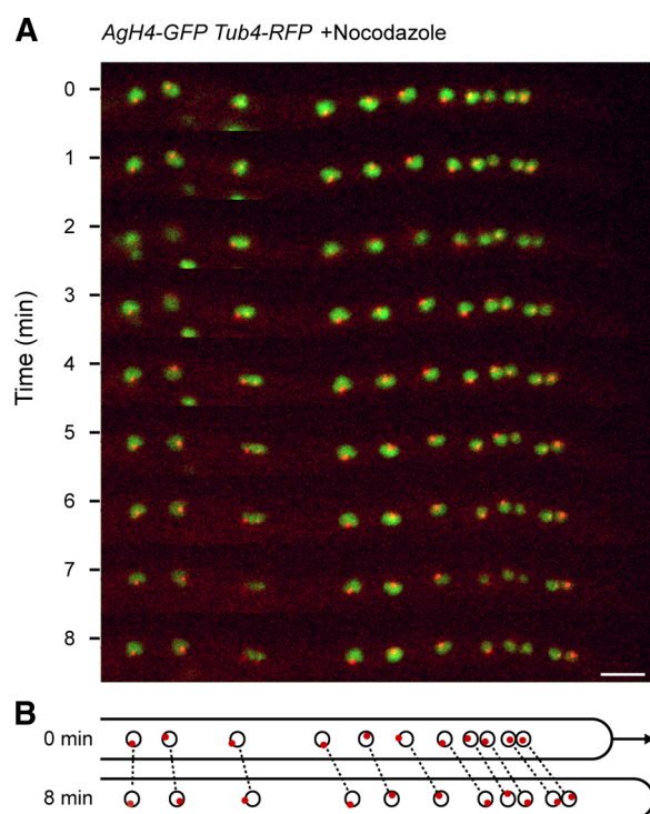
Figure 3. Migration of nuclei in the absence of cMTs. The strain expressing AgH4-GFP (green) and AgTub4-RedStar2 (red) was pre-incubated in the presence of 15 \mu\text{g}/\text{ml} nocodazole for 20 min and mounted for fluorescence videomicroscopy on agar slices containing the same concentration of nocodazole. GFP and RFP fluorescence was imaged for 500 ms each in three Z-planes, 0.75 \mu\text{m} apart, at 30-s intervals and processed (Supplemental Movie S2). (A) Nine maximal projections of Supplemental Movie S2 at 1-min intervals showing 11 evenly moving nuclei with SPBs only rarely oriented in the direction of migration. Bar, 5 \mu\text{m} . (B) Diagram of positions of nuclei (circles) and orientation of SPBs (red dots) at 0 and 8 min. Identical nuclei are connected by dotted lines. The arrow marks the elongation of the hypha within 8 min.
