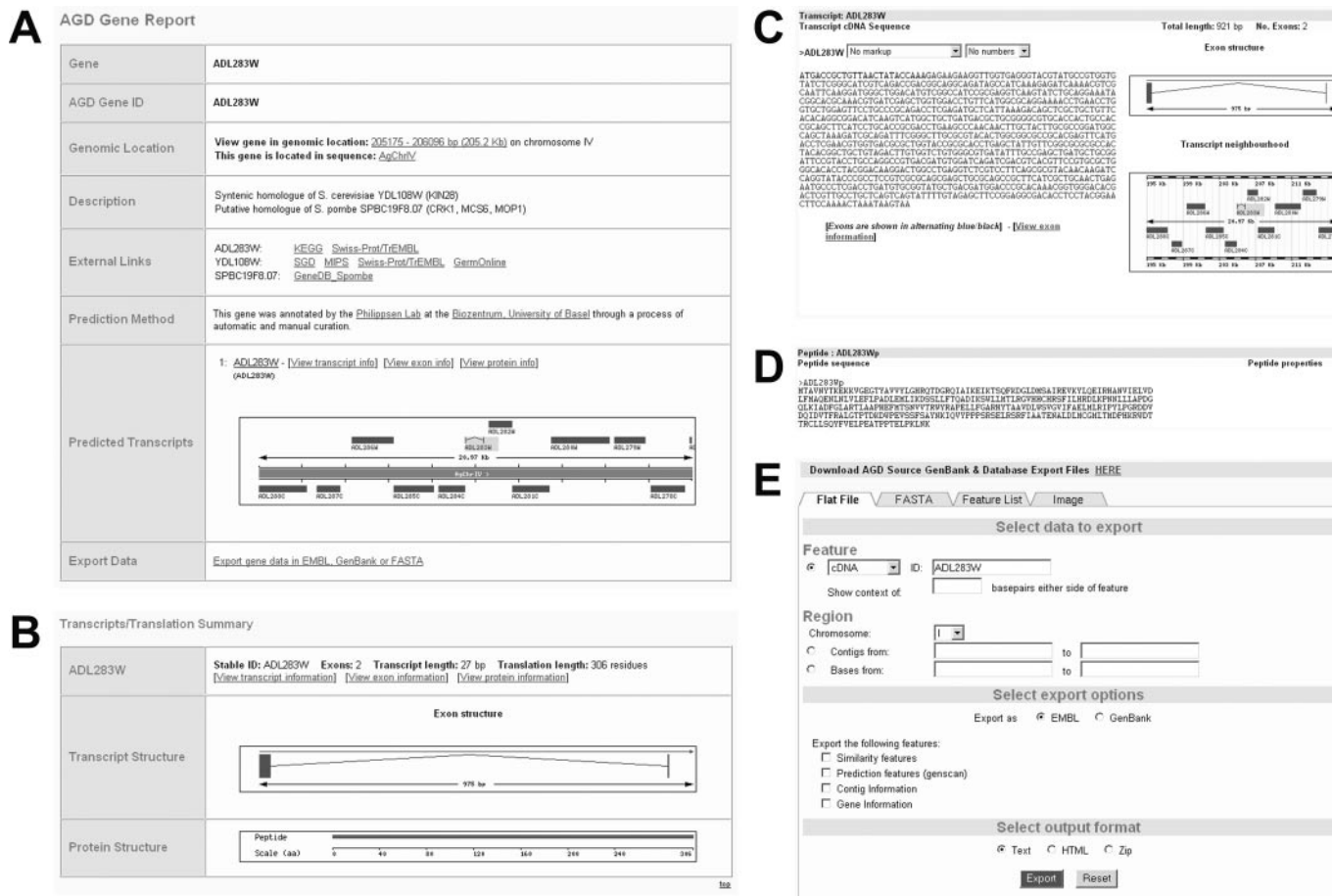
Figure 2. The locus report page of AGD. (A and B) The Gene Report and Transcript/Translation sections of the Gene Report page for the A.gossypii homolog of KIN28 ( S.cerevisiae ) and SPBC19F8.07 ( S.pombe ). (C and D) Examples of the Transcript and Peptide view, and (E) the data ExportView interface that is accessible via links in the welcome page and each Gene Report page.
