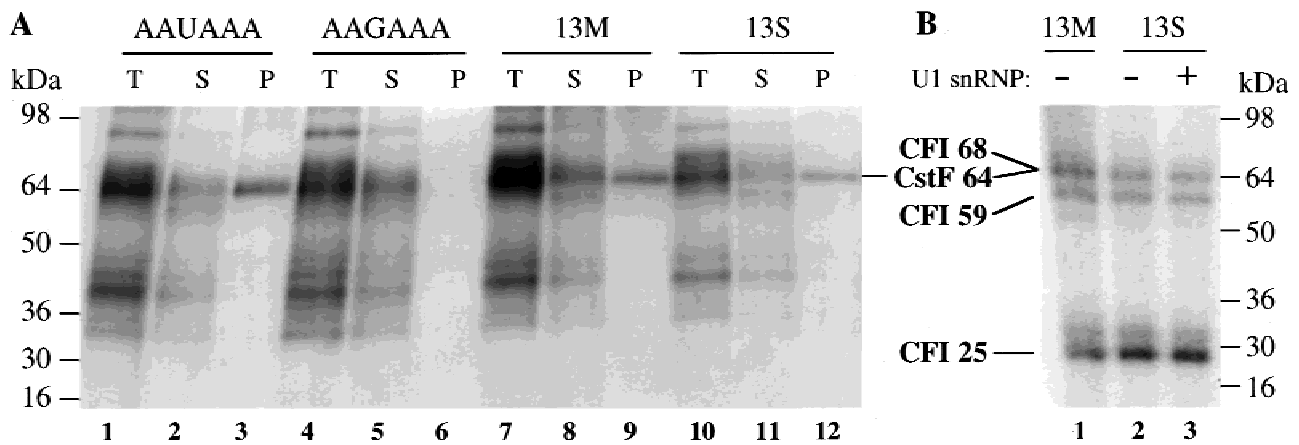
FIGURE 4. U1 snRNP does not impair the binding of CstF 64 or the CF I m subunits to the RNA. A: UV crosslinking/immunoprecipitation experiment with the 64-kDa subunit of CstF. wild-type (AAUAAA) or mutant (AAGAAA) Adenovirus L3 cleavage/polyadenylation site-containing pre-mRNAs (lanes 1–6) or the pre-mRNAs described in Figure 1 (lanes 7–12) were incubated in HeLa cell nuclear extract, crosslinked by UV irradiation, and crosslinked polypeptides were immunoprecipitated using the 3A7 monoclonal antibody directed against the 64-kDa subunit of CstF. Five percent of the crosslinked sample before immunoprecipitation (T) and the full supernatant (S) and pellet (P) fractions after immunoprecipitation were resolved by 10% SDS-PAGE. Protein markers are indicated on the left. B: UV crosslinking experiment with CF I m . The different RNA substrates were incubated with the purified cleavage/polyadenylation components (as in Fig. 3) in the absence (lanes 1–2) or the presence (lane 3) of 200 ng purified U1 snRNP, crosslinked by UV irradiation, and loaded on a 10% SDS-PAGE gel. The position and nature of the crosslinked proteins (64-kDa subunit of CstF and the 68-, 59-, and 25-kDa subunits of CF I m ) are shown on the left, protein markers on the right.
