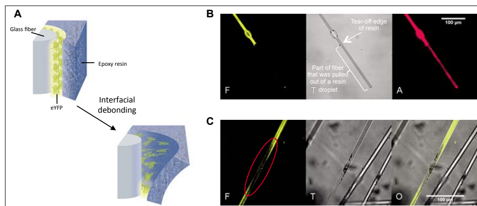
Fig. 4. A) Fluorescent protein acting as a mechanophore at the fiber-resin interface in fiber-reinforced composites. Interfacial debonding defects cause mechanical unfolding of the protein and thereby a loss of the protein's fluorescence. B) Confocal fluorescence image of eYFP on a glass fiber after fiber pullout from a microdroplet of epoxy resin. The fiber was immunostained with an Alexa Fluor 647-antibody in order to detect native and unfolded eYFP. (Channels: F = eYFP, T = transmission, A = Alexa Fluor 647); C) Confocal microscopy image of an eYFP/glass fiber/epoxy resin composite after having been subjected to low velocity impact. Diminished fluorescence in the vicinity of a fiber fracture is marked by a red oval. (Channels: F = eYFP, T = transmission, O = overlay) Adapted with permission from ref. [4]. Copyright 2013 Wiley-VCH Verlag GmbH & Co. KGaA.
