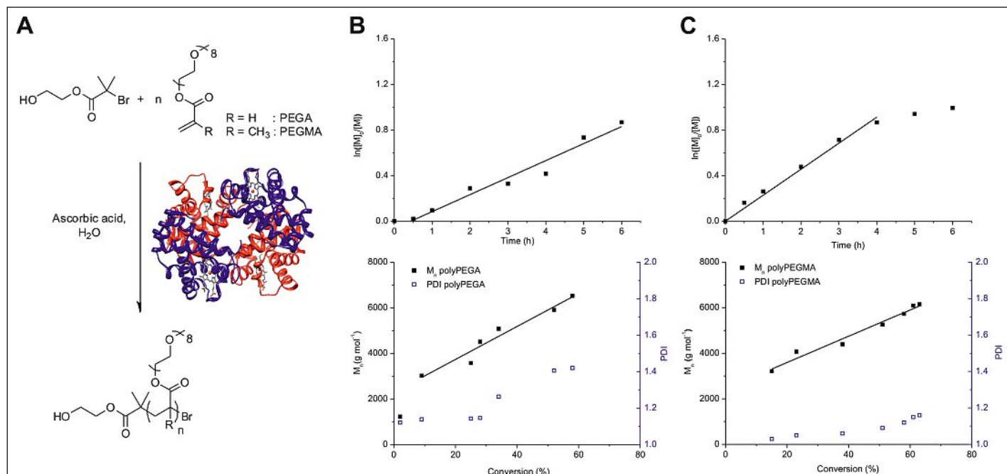
Fig. 1. A) ARGET ATRP of water-soluble monomers catalyzed by Cys-blocked hemoglobin. B, C) First order kinetic plots, and molecular weight and polydispersity as a function of conversion: (B) PEGA, (C) PEGMA. Adapted with permission from ref. [2c]. Copyright 2013 American Chemical Society.
