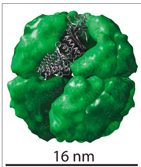
Fig. 3. The protein cage thermosome from Thermoplasma acidophilum is explored as a nanoreactor. Adapted with permission from ref. [14a]. Copyright 2011 Wiley-VCH Verlag GmbH & Co. KGaA.
