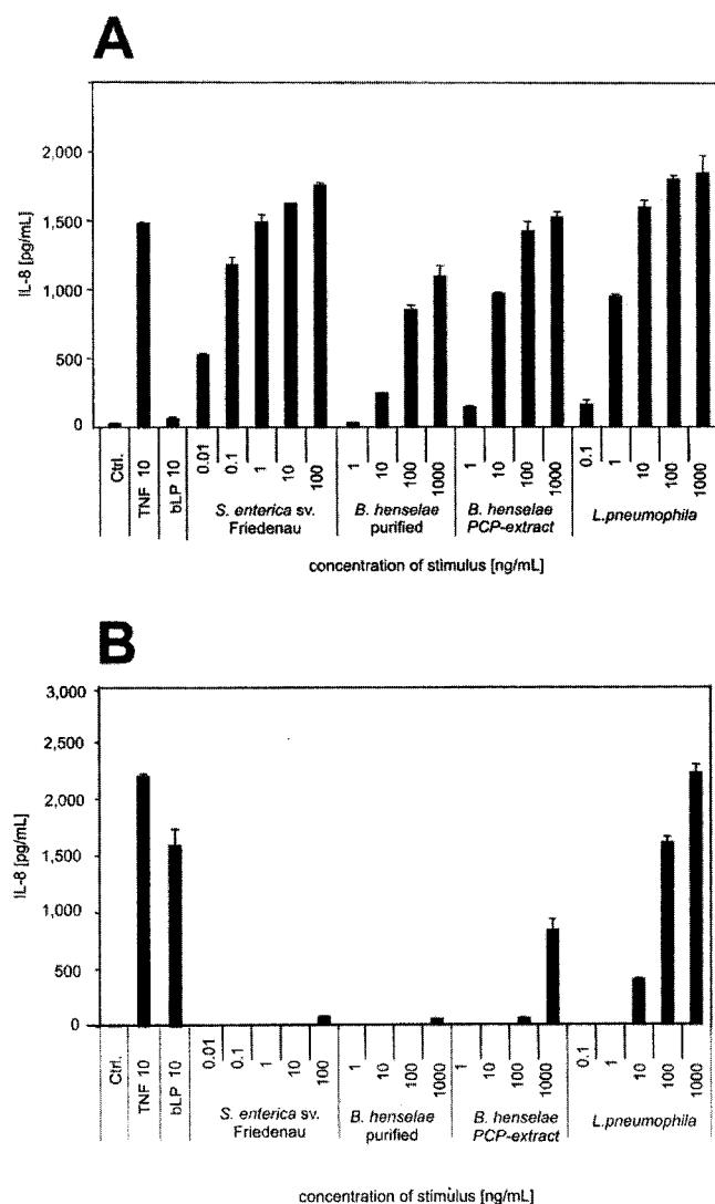
FIG. 7. Purified LPS from B. henselae ATCC 49882 T activates HEK293 cells through TLR-4/MD-2. HEK293 cells were transiently transfected with CD14 and either TLR4/MD-2 (A) or TLR2 (B) as described under "Experimental Procedures." After 24 h, cells were stimulated with indicated ligands for 18 h. Interleukin-8 content of the supernatant was analyzed by enzyme-linked immunosorbent assay. One representative experiment out of three is shown.
