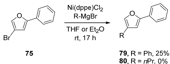
Scheme 2.16 Synthesis of 2,4-disubstituted furans.
