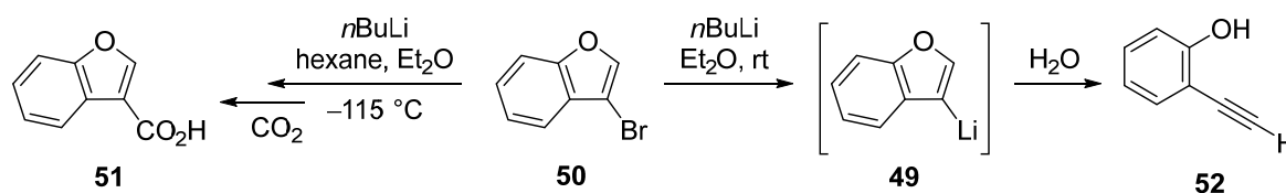
Scheme 2.5 Generation of 3-lithiobenzofuran ( 49 ).
