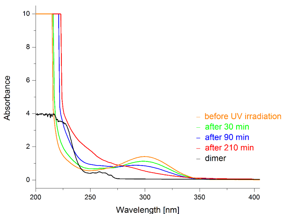
Figure 5.2 Irradiation of 2,5-dibenzylthiophene 1,1-dioxide ( 141 ) with a Xe lamp in CH 3 CN.
