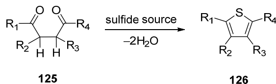
Scheme 4.2 Synthesis of thiophenes via cyclization reactions.
