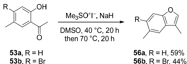
Scheme 2.20 Synthesis of 3-substituted benzofurans by COREY-CHAYKOVSKY reaction.
