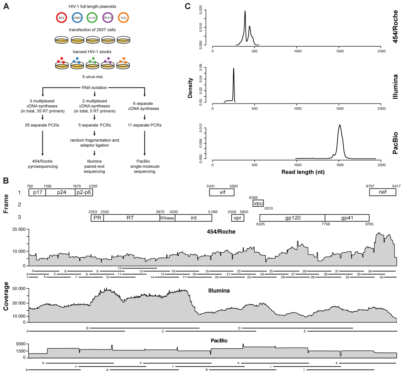
Figure 1. HIV-1 full-length genome sequencing using three different NGS technologies. (A) Experimental protocol. Five HIV-1 full-length plasmids were transfected into 293T cells to generate five different virus stocks. These clones were mixed in a large batch and aliquoted. RNA was isolated and amplified with three different protocols. DNA libraries were sequenced with either 454/Roche, Illumina or PacBio. (B) Coverage in overlapping reads per base pair. The map of the HIV-1 genome is shown on the top, with each subsequently analyzed gene indicated. The position numbering refers to the HIV-1 HXB2 genome (GenBank accession number K03455). Amplicon layout is visualized for each NGS platform with individual numbering (Supplementary Table S1). (C) Read length distribution of each NGS technology, after preprocessing and alignment.
