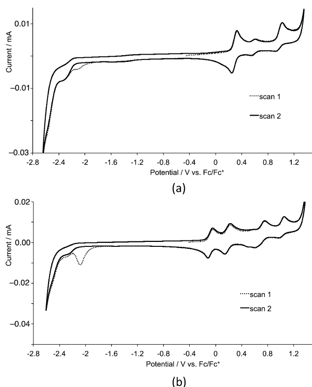
Fig. 10 Cyclic voltammograms of CH 2 Cl 2 (degassed) solutions of (a) [Cu(3) 2 ][PF 6 ] and (b) [Cu(9) 2 ][PF 6 ] for first- and second cycles. Scan rate = 0.1 V s -1 .
