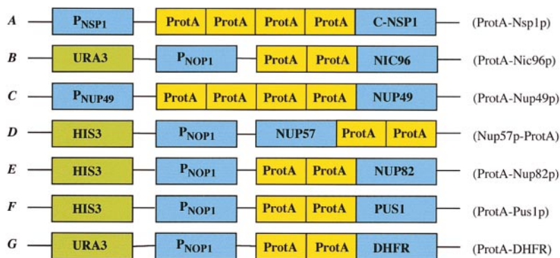
Figure 2. Schematic diagram of the fusion constructs used in this study: (A) Four IgG-binding domains derived from S. aureus protein A (ProtA) and the essential NSP1 COOH-terminal domain. (B) Two IgG-binding domains of ProtA and the NIC96 gene under control of the NOP1 promoter and URA3 selection. (C) Four IgG-binding domains of ProtA and the NUP49 gene. (D) Two IgG-binding domains of ProtA and the NUP57 gene under control of the NOP1 promoter and HIS3 selection. (E) Two IgG-binding domains of ProtA and the NUP82 gene under control of the NOP1 promoter and HIS3 selection. (F) Two IgG-binding domains of ProtA and the PUS1 gene under control of the NOP1 promoter and HIS3 selection. (G) Two IgG-binding domains of ProtA and the DHFR gene under control of the NOP1 promoter and URA3 selection.
