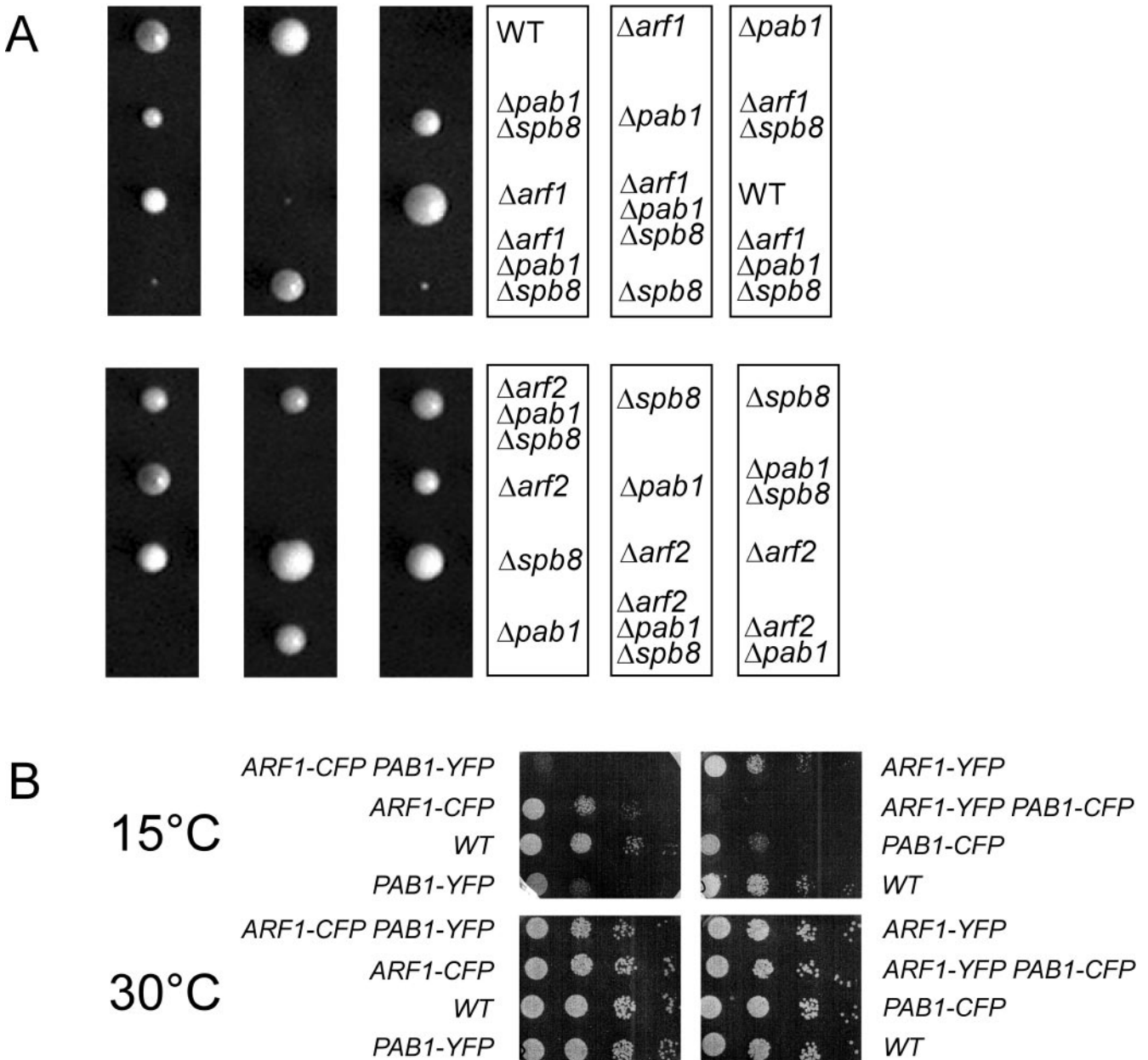
Figure 2. ARF1 but not ARF2 interacts genetically with PAB1 . (A) \Delta arf1 or \Delta arf2 haploid strains were crossed with \Delta pab1\Delta spb8 strains. The resulting diploid or tetrads were sporulated and tetrads dissected. The spores were grown for 2 d at 30°C. (B) ARF1 and PAB1 were chromosomally appended with either yellow fluorescent protein (YFP) or cyan fluorescent protein (CFP). The resulting strains were grown to early log phase, and serial dilutions were spotted on YPD plates. The plates were incubated at the indicated temperatures.
