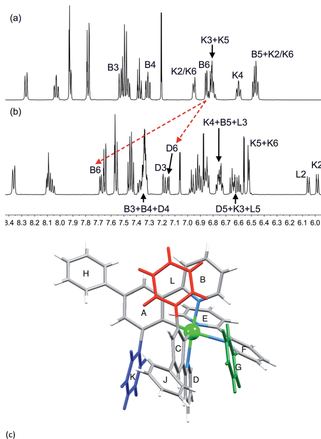
Fig. 6 500 MHz ^1\text{H} NMR spectrum (295 K, \text{CD}_2\text{Cl}_2 ) of (a) [\text{Ir}(\text{Ph}_2\text{ppy})_2(1)]^+[\text{PF}_6]^- and (b) [\text{Ir}(\text{Ph}_2\text{ppy})_2(2)]^+[\text{PF}_6]^- . Chemical shifts in \delta/\text{ppm} . (c) Structure of [\text{Ir}(\text{Ph}_2\text{ppy})_2(2)]^+ (from the solid-state determination) showing rings G, K and L.
