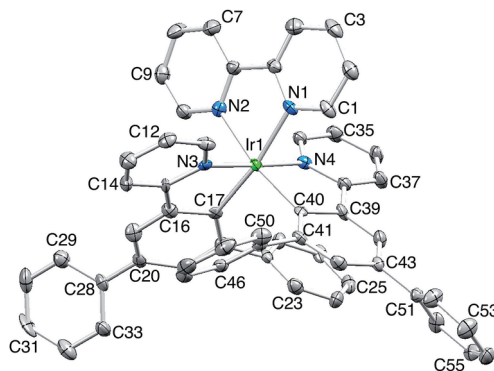
Fig. 2 The structure of the \Lambda - [\text{Ir}(\text{Ph}_2\text{ppy})_2(\mathbf{1})]^+ cation in racemic [\text{Ir}(\text{Ph}_2\text{ppy})_2(\mathbf{1})][\text{PF}_6] \cdot \text{EtOH} (H atoms omitted, ellipsoids plotted at 40% probability). Selected bond parameters: \text{Ir1}-\text{C17} = 2.027(9) , \text{Ir1}-\text{N3} = 2.043(9) , \text{Ir1}-\text{C40} = 2.052(9) , \text{Ir1}-\text{N4} = 2.078(8) , \text{Ir1}-\text{N1} = 2.125(8) , \text{Ir1}-\text{N2} = 2.152(7) Å; \text{N1}-\text{Ir1}-\text{N2} = 76.7(3) , \text{C17}-\text{Ir1}-\text{N3} = 80.9(3) , \text{C40}-\text{Ir1}-\text{N4} = 81.5(3)^\circ .
