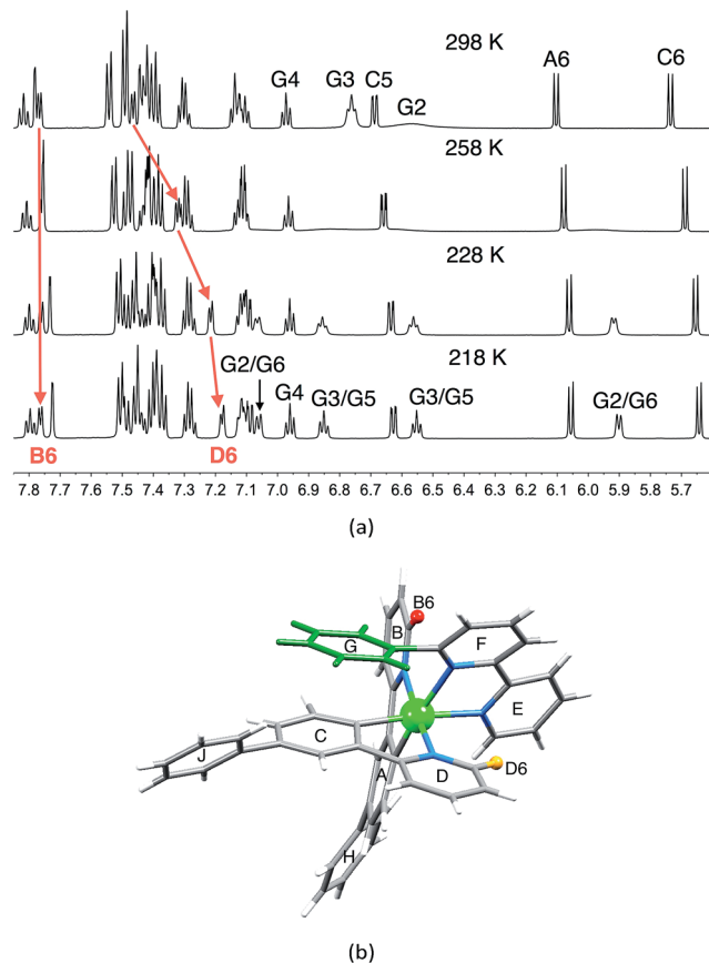
Fig. 5 (a) Part of the 600 MHz ^1\text{H} variable temperature NMR spectra of a \text{CD}_2\text{Cl}_2 solution of [\text{Ir}(\text{Phppy})_2(2)]^+[\text{PF}_6]^- ; the full spectrum is shown in Fig. S5.† (b) Modelled structure of [\text{Ir}(\text{Phppy})_2(2)]^+ with protons \text{H}^{\text{B6}} and \text{H}^{\text{D6}} and the phenyl (G) ring highlighted.
