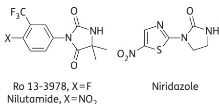
Figure 1. Structures of Ro 13-3978, nilutamide and niridazole.
