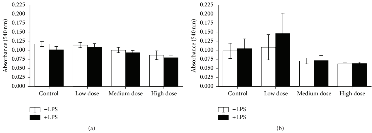
FIGURE 9: NR test after the NO test in trunk kidney cells. Cell vitality after 96 h of in vitro culture of trunk kidney cells of fish after 4 weeks of feeding ZEN (a) and with additional 2 weeks of recovery (b) assayed by means of uptake of neutral red measured by absorption at 540 nm, n = 6 ; mean \pm SEM; difference to controls at P < 0.05 .
