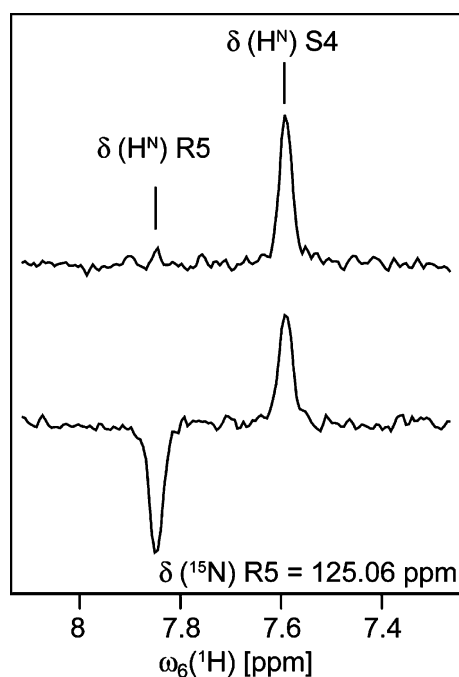
Figure 3. Suppression of the C_{i-1}^{\alpha} \rightarrow {}^{15}N_i back transfer (Figure 1) in the 6D-APSY-seq-HNCOCANH spectrum of [^{13}C, ^{15}N] -labeled 434-repressor(1–63) (protein concentration = 0.9 mM, 20 mM sodium phosphate at pH 6.5, T=15^{\circ}C ). Shown are 1D cross sections through the projection spectra recorded with the projection angles (\alpha, \beta, \gamma, \delta) = (0^{\circ}, 90^{\circ}, 0^{\circ}, 0^{\circ}) , which were taken at the Arg 5 {}^{15}N -frequency of 125.06 ppm and cover the {}^1H^N chemical shift range containing the intraresidual correlation to Arg 5 and the sequential correlation to Ser 4. The time period T = t_4^a + t_4^b + t_4^c (Figure 2) was set to 50 ms (top) and 27 ms (bottom), resulting in experiments with (top) and without (bottom) suppression of back transfer.
