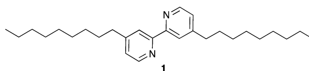
Scheme 1 Structure of ligand \mathbf{1} . See Scheme S1 (ESI†) for the structure of [\text{Ru}(\mathbf{1})_3]^{2+} .
