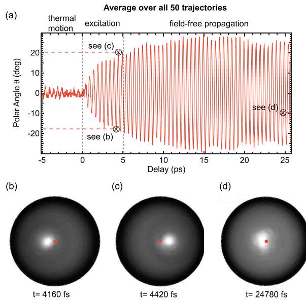
FIG. 4. Simulation of a THz pump-XPD probe measurement. In (a), the time-dependent polar angle of maximum emission from the averaged diffraction maps is plotted. It represents the ensemble-averaged orientation of the CO molecules on Pt(111). For positive delays, an oscillation with \nu = 2.0 THz is visible. At delays between the dashed lines the pump pulse is present. (b)–(d) The averaged diffraction maps that were calculated with SSC simulations. No normalization was applied. The delay times of all three patterns are marked in (a) with black circles. Each diffraction map is ensemble averaged over calculations from 50 different cluster files. The red dots in the center of the maps show the normal emission direction.
