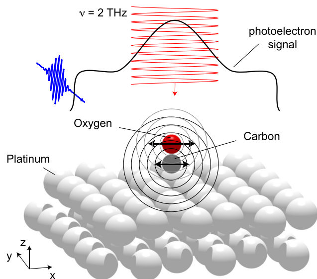
FIG. 1. Sketch of the pump-probe experiment to record time-resolved XPD data. The 2 THz pulse (red) acts as pump pulse and the CO molecule on top of the Pt(111) surface follows the field of the THz radiation (black arrows). With the (blue) x-ray pulse the molecular orientation is probed by recording an XPD pattern. The unscattered C 1s photoelectron wave is indicated by solid circles, the wave scattered off the oxygen atom by light grey circles. The solid curve above the surface illustrates the resulting C 1s intensity distribution. Note: The wavelength of the 2 THz pulse is much larger ( \lambda \approx 150 \mu\text{m} ) than shown here.
