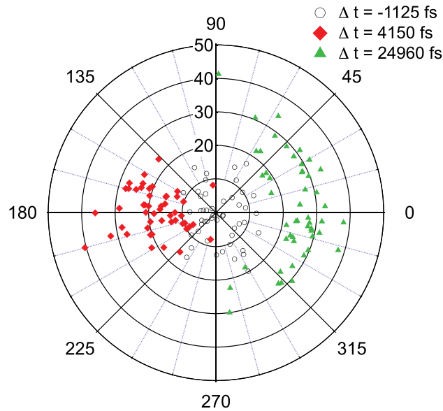
FIG. 6. Angular order of the CO molecules. At three different times, the angular position ( \theta, \phi ) of the oxygen atom with respect to the carbon emitter is plotted for each of the 50 trajectories: before the THz pulse (black), near the end of the pulse (red) and 20 ps after the pulse (green).
