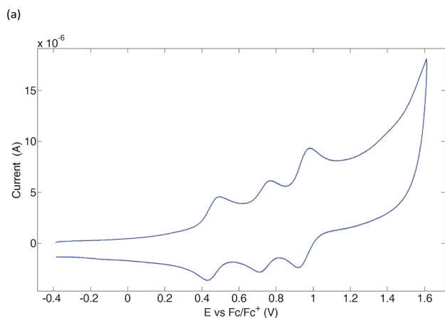
Fig. 4 Oxidation processes in the cyclic voltammograms of (a) 3 and (b) [\text{Ru}(\text{3})(\text{4})][\text{PF}_6]_2 . For conditions, see Table 1.
