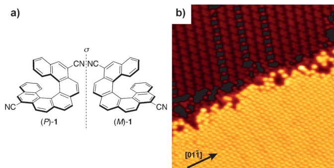
Figure 1. a) Molecular structures of the two enantiomers of 6,13-dicyano-7]helicene, ( P )- 1 and ( M )- 1 . b) Overview STM image (43 × 43 nm 2 , 77 K) of ( P )- 1 , showing a dimeric (bottom) next to a tetrameric (top) arrangement. Note that a Cu step edge runs from the lower left to the upper right.
