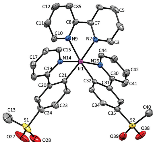
Fig. 3 Structure of one of the independent \Lambda -[Ir(2) 2 (bpy)] + cations in the asymmetric unit in 2{[Ir(2) 2 (bpy)]PF 6 }·5.5H 2 O; ellipsoids are plotted at the 40% probability level and H atoms, [PF 6 ] − counterion and solvent molecules are omitted for clarity. Selected bond lengths and angles: Ir1–N2 = 2.134(4), Ir1–N9 = 2.134(4), Ir1–N14 = 2.045(4), Ir1–N29 = 2.045(4), Ir1–C21 = 2.000(4), Ir1–C32 = 2.006(4), S1–C13 = 1.719(10), S1–O27 = 1.454(6), S1–O28 = 1.415(5), S2–O38 = 1.431(4), S2–O39 = 1.431(4), C40–S2 = 1.761(6) Å; N2–Ir1–N9 = 76.72(16), N14–Ir1–C21 = 80.67(16), N29–Ir1–C32 = 80.61(16), N14–Ir1–N29 = 172.70(14), N2–Ir1–C21 = 175.99(16), N9–Ir1–C32 = 173.13(16), O27–S1–O28 = 114.8(4), O38–S2–O39 = 117.5(3)°.
