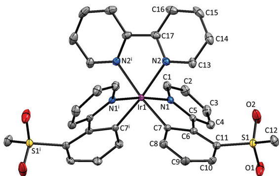
Fig. 4 Structure of the \Lambda -[Ir(3) 2 (bpy)] + cation in [Ir(3) 2 (bpy)]PF 6 ; ellipsoids are plotted at the 40% probability level and H atoms and [PF 6 ] − counterion are omitted for clarity. Symmetry code: i = 1 - x, y, \frac{1}{2} - z . Selected bond lengths and angles: Ir1–N1 = 2.036(2), Ir1–N2 = 2.146(2), Ir1–C7 = 2.007(2), S1–O1 = 1.432(2), S1–O2 = 1.433(2), C12–S1 = 1.763(3) Å; N1–Ir1–C7 = 80.08(9), N2–Ir1–N2 i = 76.83(11), N2–Ir1–C7 i = 173.07(9), N1–Ir1–N1 i = 173.67(11), O1–S1–O2 = 118.38(18)°.
