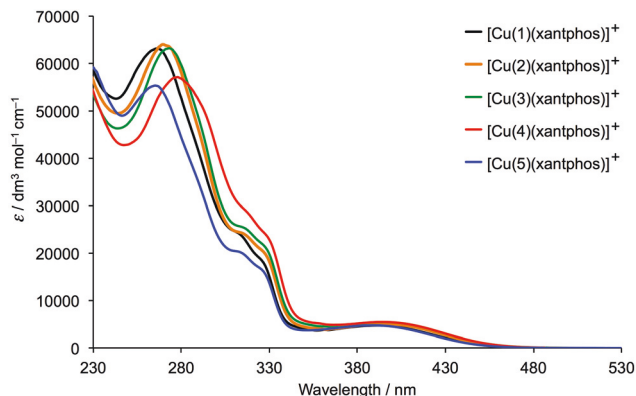
Fig. 9 Solution ( \text{CH}_2\text{Cl}_2 , 2.5 \times 10^{-5} \text{ mol dm}^{-3} ) absorption spectra of [\text{Cu}(\text{N}^{\wedge}\text{N})(\text{xantphos})][\text{PF}_6] ( \text{N}^{\wedge}\text{N} = 1-5 ).
