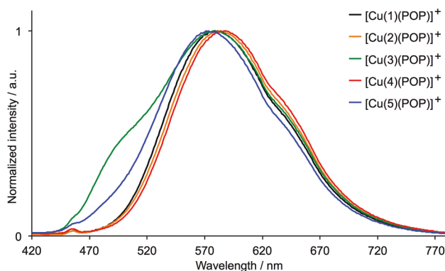
Fig. 10 Normalized solution ( \text{CH}_2\text{Cl}_2 , 2.5 \times 10^{-5} \text{ mol dm}^{-3} ) emission spectra of [\text{Cu}(\text{N}^{\wedge}\text{N})(\text{POP})][\text{PF}_6] ( \lambda_{\text{exc}} = 400 \text{ nm} , see Table 2 for \lambda_{\text{em}}^{\text{max}} ).
