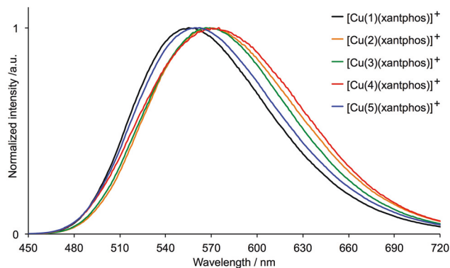
Fig. 11 Normalized solid-state emission spectra of [\text{Cu}(\text{N}^{\wedge}\text{N})(\text{xantphos})][\text{PF}_6] ( \text{N}^{\wedge}\text{N} = 1-5 ) ( \lambda_{\text{exc}} = 365 \text{ nm} ).
