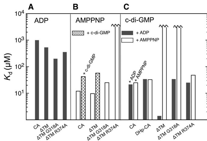
Fig. 3. Ligand binding to various CckA constructs. K_d determination was measured by isothermal titration calorimetry (ITC). (A) ADP. (B) AMPPNP in the absence or presence of 100 \mu M c-di-GMP. (C) c-di-GMP in the presence of 5 mM ADP or AMPPNP. Further information is given in table S2 and fig. S4.
