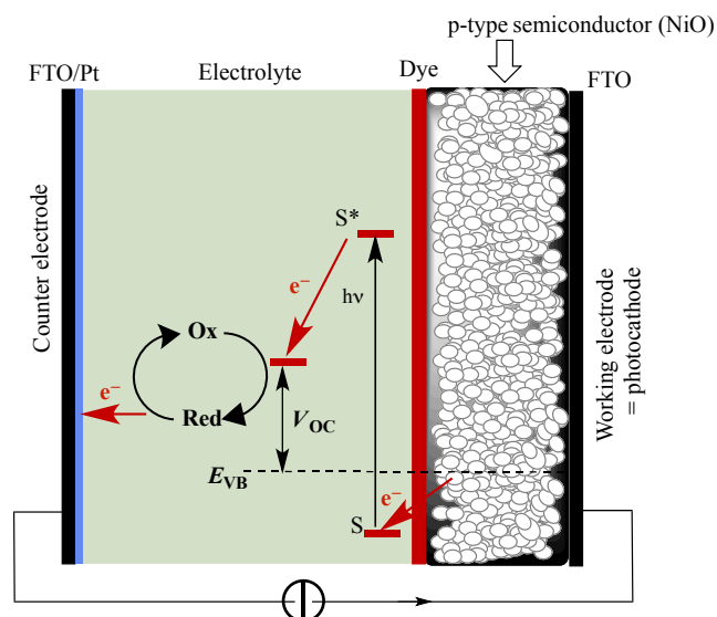
Fig. 1. Working principle of a p-type DSC. S and S* are the ground and excited states of the dye; E_{\text{VB}} represents the quasi-Fermi level of the valence band of the semiconductor; V_{\text{OC}} = open circuit voltage.
