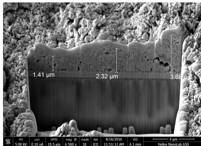
Fig. 7. FIB images of an FTO/NiO electrode with [\text{Ni}(\text{acac})_2] pretreatment and two screen-printed layers of NiO sintered at 350 °C: (a) top surface, and (b) a gallium beam cut into the NiO with a platinum layer is deposited on top of the NiO surface. In (b), the glass and FTO coating are visible beneath the NiO.
