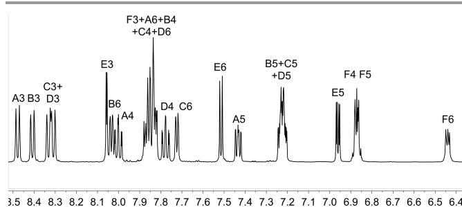
Fig. 2. The 500 MHz ^1\text{H} NMR spectrum of [\text{Ru}(\text{bpy})_2(\mathbf{1})][\text{PF}_6] (in \text{CD}_3\text{CN} ). Atom labels are given in Scheme 3.
