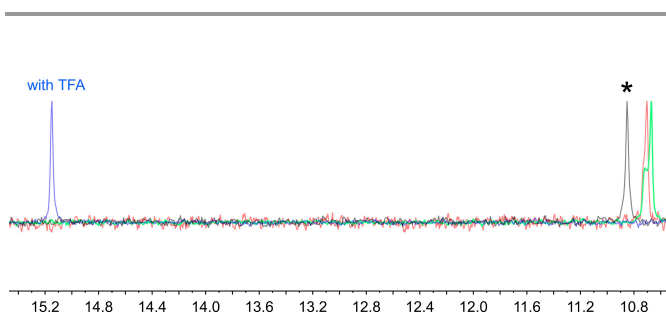
Fig. 5. 162 MHz ^{31}\text{P}\{^1\text{H}\} NMR spectrum of [\text{Ru}(\text{bpy})_2(\text{H5})] (*) in \text{CD}_3\text{OD} , and spectra taken after the addition of (a) \text{CF}_3\text{CO}_2\text{H} (TFA, blue), (b) \text{K}_2\text{CO}_3 (green) or (c) \text{CF}_3\text{CO}_2\text{H} followed by \text{K}_2\text{CO}_3 (red).
