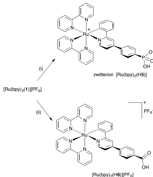
Scheme 5. Conversion of [Ru(bpy) 2 (1)][PF 6 ] to [Ru(bpy) 2 (H5)] and [Ru(bpy) 2 (H6)][PF 6 ]. Optimized conditions: (i) H 2 4, K 3 PO 4 , SPhos Pd G2, MeCN/H 2 O; 70 °C, 5 h; (ii) 4-carboxyphenylboronic acid, K 3 PO 4 , SPhos Pd G2, MeCN/H 2 O; 70 °C, 5 h.
