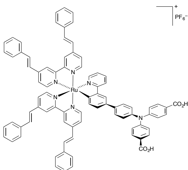
Scheme 7. Structure of a cyclometallated ruthenium dye that achieves J_{sc} = 3.43 mA cm -2 and \eta = 0.104\% . 9
