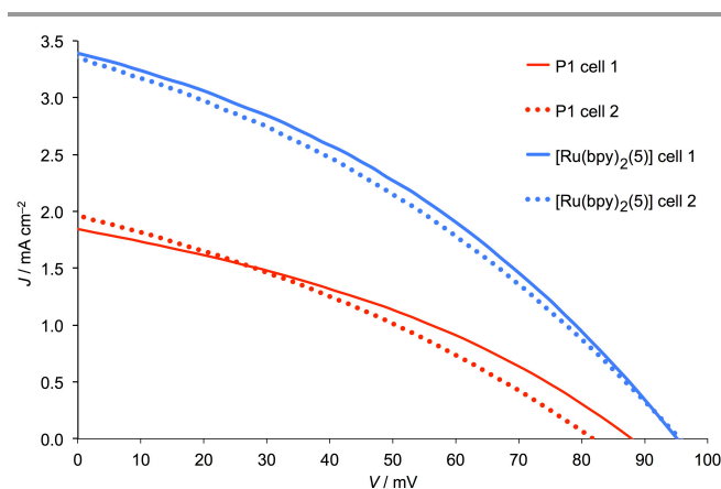
Fig. 9. J - V curves for duplicate DSCs containing dyes P1 and [Ru(bpy) 2 (H5)].
