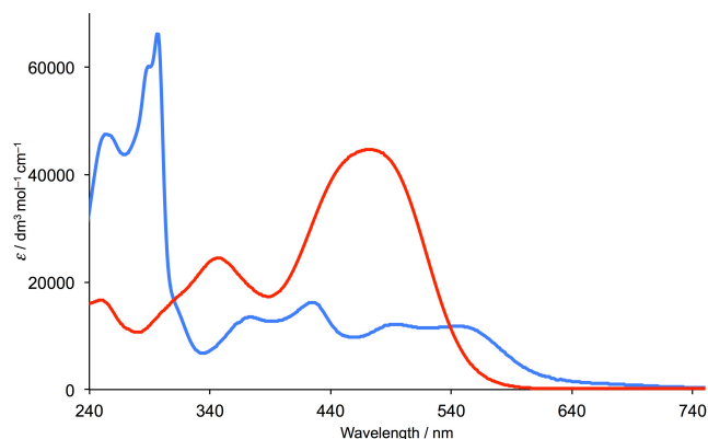
Fig. 6. The solution absorption spectra of [\text{Ru}(\text{bpy})_2(\text{H5})] (MeOH, 1 \times 10^{-5} mol \text{dm}^{-3} , blue curve) and of the dye P1 (MeCN, 1 \times 10^{-5} mol \text{dm}^{-3} , red curve).
