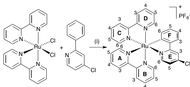
Scheme 3. Cyclometallation reaction to form [\text{Ru}(\text{bpy})_2(\mathbf{1})][\text{PF}_6] . Conditions: (i) \text{AgPF}_6 , \text{CH}_2\text{Cl}_2 , reflux, 19 h. Ring and atom labels used for NMR assignments are shown.
