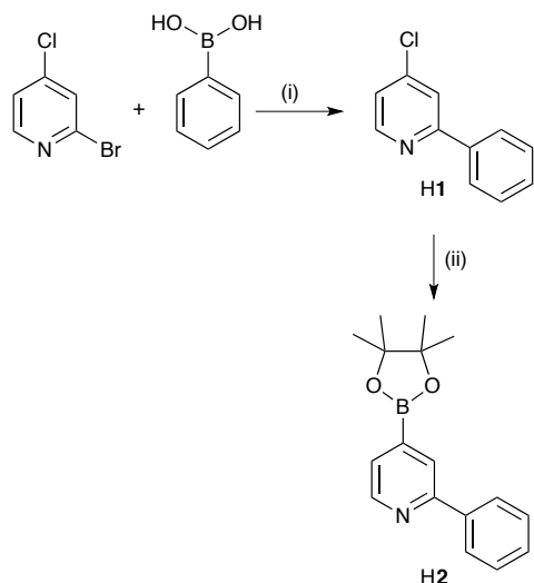
Scheme 2. Syntheses of intermediates H1 and H2. Conditions: (i) \text{Na}_2\text{CO}_3 , [\text{Pd}(\text{PPh}_3)_2\text{Cl}_2] , \text{THF}/\text{H}_2\text{O} , 60 °C, 3h; (ii) bis(pinacolato)diboron, KOAc, [\text{Pd}(\text{dppf})\text{Cl}_2] , dioxane, reflux, 72 h.
