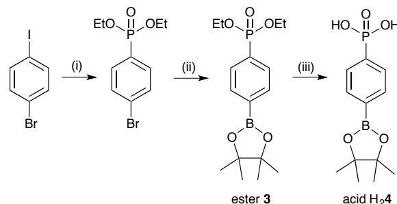
Scheme 4. Synthesis of the phosphonic acid building block 4 . Conditions: (i) HPO(OEt) 2 , Cs 2 CO 3 , [Pd(PPh 3 ) 4 ], THF, reflux, 2.5 h; (ii) bis(pinacolato)diboron, KOAc, [Pd(dppf)Cl 2 ], THF, microwave reactor, 90 °C, 1 h; (iii) Me 3 SiBr, CH 2 Cl 2 , room temperature, 19 h.
