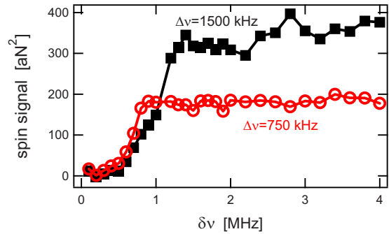
FIG. 3. (Color online) Spin signal as a function of rf frequency separation for the case of excitation at two rf frequencies. Points show the force-detected spin signal measured for \nu_1=114 MHz in the presence of a second rf excitation that is offset in frequency by \delta\nu . Results for two FM modulations \Delta\nu are shown.
