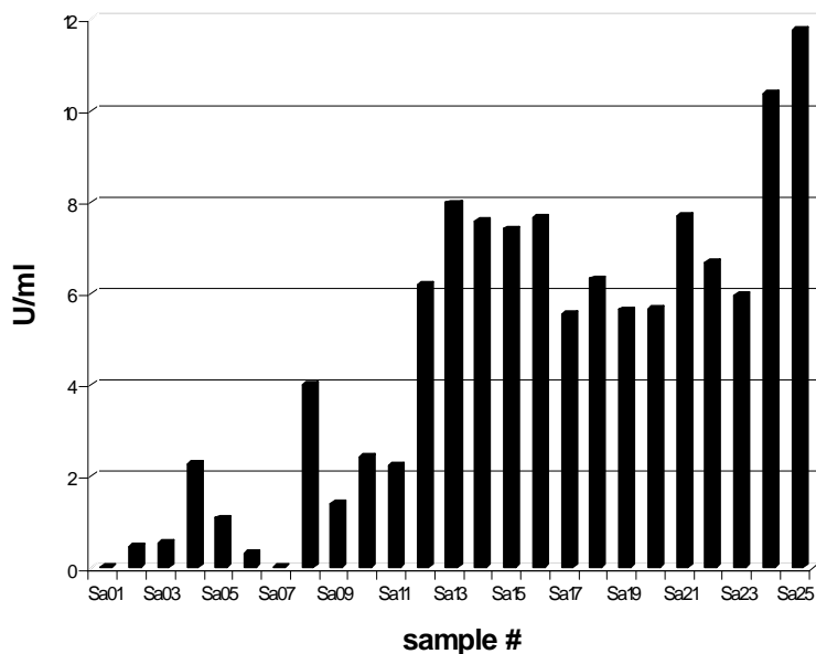
Figure 13. The mean result of PY ShcA detection in 25 samples after fitting the standard curve.
