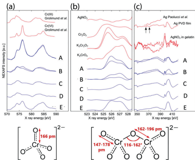
Fig. 3 STXM spectra. (a) Cr L_{3,2} edges, (b) O K edge and (c) Ag M edge average spectra (blue curves) of 10 square areas of 20 \text{ nm} \times 20 \text{ nm} on the fine structure of a large band (A), background between the fine structure in the band (B), on the fine structure between bands (C) and background where no precipitation occurred (D). Spectra E were taken on a band in a pattern which only contained the large bands. As references (red curves) for (a) we added Cr(III) and Cr(VI) spectra from ref. 20, for (b) we acquired \text{K}_2\text{Cr}_2\text{O}_7 , \text{K}_2\text{CrO}_4 and \text{AgNO}_3 spectra and used \text{Cr}_2\text{O}_3 spectrum from ref. 21. For references for the silver edge spectra (c) we used \text{AgNO}_3 in a gelatin film, our physical vapor deposited Ag film and a polycrystalline Ag sample. 22 Structural properties of the chromate and dichromate anions were taken from ref. 23.
