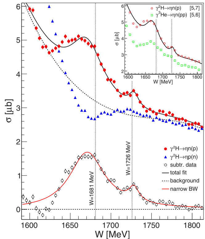
FIG. 1. (Color online) Excitation functions for quasifree photoproduction of \eta mesons. Inset: total cross sections for quasifree neutrons bound in the deuteron (red circles) and in {}^3\text{He} nuclei (green squares). Data are as published in Fig. 1 of Ref. [5]. Fit curves include Breit-Wigner resonance for the structure at 1726 MeV. Main figure: finer binned data for the measurement with deuterium target. Red circles (blue triangles): quasifree neutron (proton) data. Curves: total fit (solid black curve), background contributions (dashed black curve), and sum of two narrow signal Breit-Wigner functions (red solid curve). Open black circles: background-subtracted neutron data. Vertical lines: markers at W = 1681 MeV and W = 1726 MeV.
