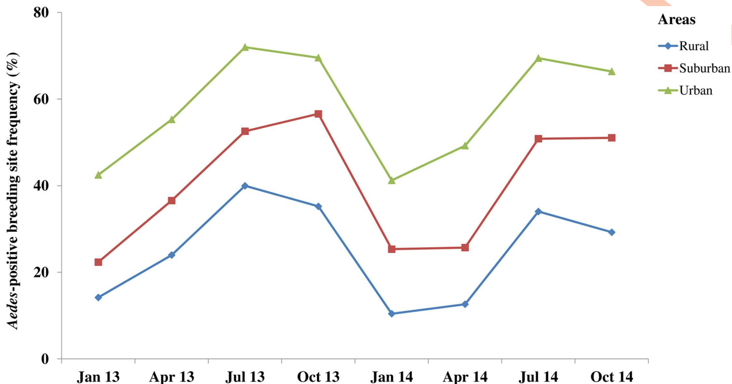
Fig 4. Monthly variations in the occurrence of immature stages of Aedes mosquitoes in rural, suburban, and urban areas in south-eastern Côte d'Ivoire.
