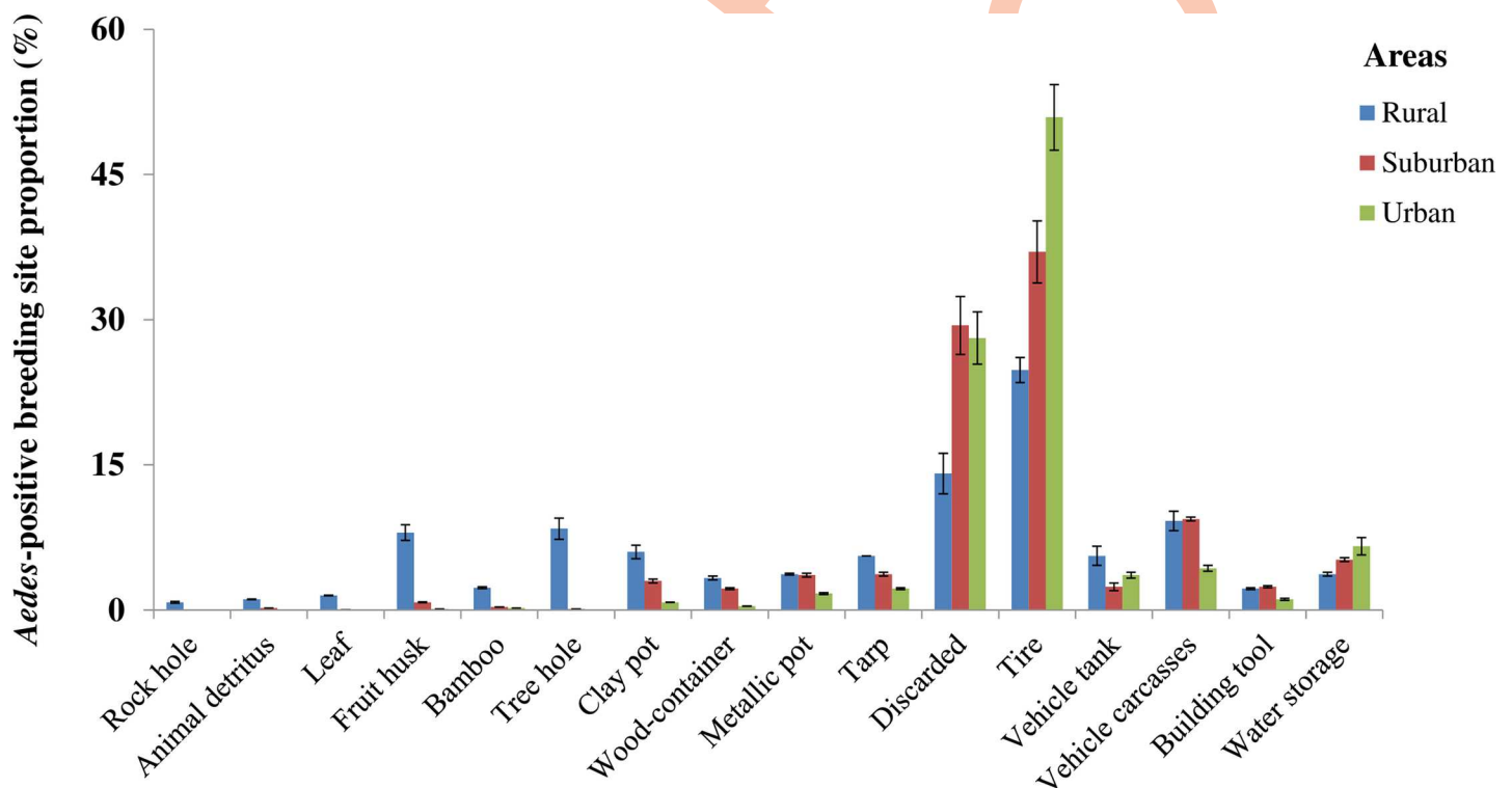
Fig 3. Frequency of Aedes mosquito breeding sites in rural, suburban, and urban areas in south-eastern Côte d'Ivoire. Error bars show the standard error (SE).
