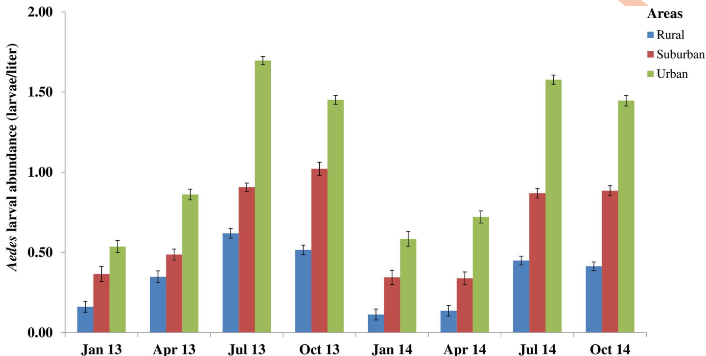
Fig 5. Monthly variations in the abundance of immature stages of Aedes mosquitoes in rural, suburban, and urban areas in south-eastern Côte d'Ivoire. Error bars show the standard error (SE).
