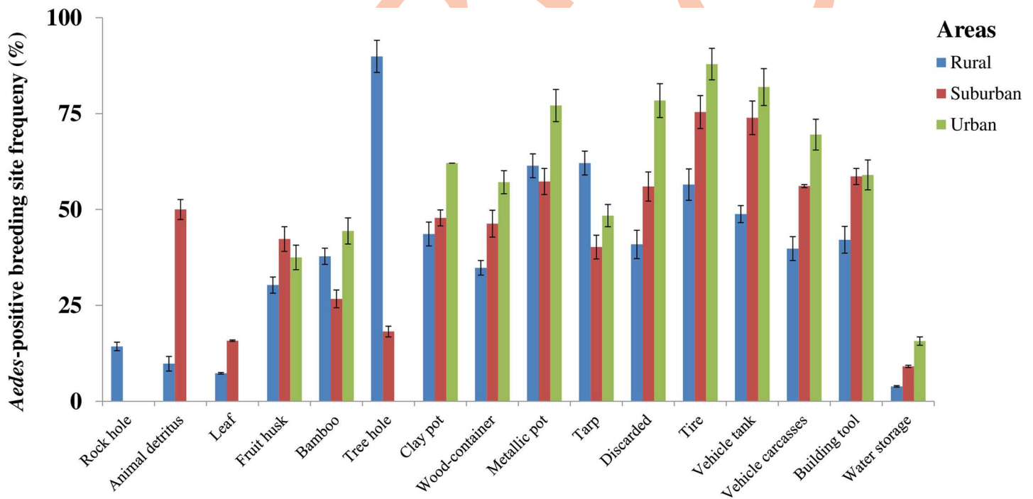
Fig 2. Dynamics of Aedes mosquito breeding sites in rural, suburban, and urban areas in south-eastern Côte d'Ivoire. Error bars show the standard error (SE).
