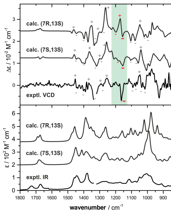
Figure 3. Comparison of the VCD (top) and IR (bottom) spectra of bifurcatriol 1 (measured in benzene- d_6 ) with those calculated for (7S,13S)-1 and (7R,13S)-1. The green shaded VCD signatures appear to be characteristic for the stereocenter at C-7. Spectral regions around 1340 \text{cm}^{-1} and below 900 \text{cm}^{-1} are left out due to solvent absorbance and high noise.
