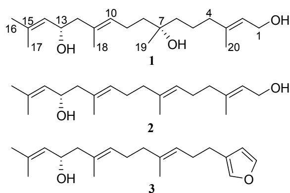
Figure 1. Structure of compounds (1–3) obtained from B. bifurcata .
