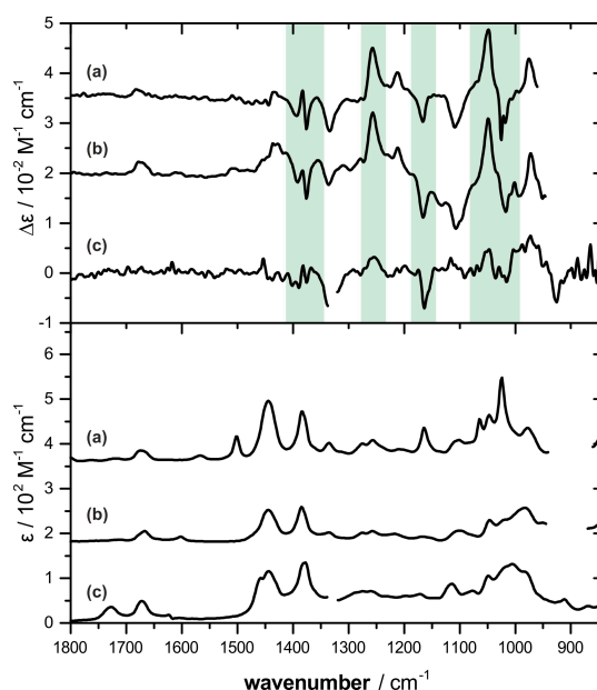
Figure 2. Comparison of the VCD (top) and IR (bottom) spectra of bifurcatriol ( 1 ) (traces c, measured in benzene- d 6 ) against elegandiol ( 2 ) (traces b, CDCl 3 ) and bifurcane ( 3 ) (traces a, CDCl 3 ) reported previously [22]. The green shaded VCD signatures appear to be characteristic for the C-13 stereocenter. Spectral regions around 1340 cm -1 (traces c) and between 950–870 cm -1 (traces a and b) are left out due to solvent absorbance.
