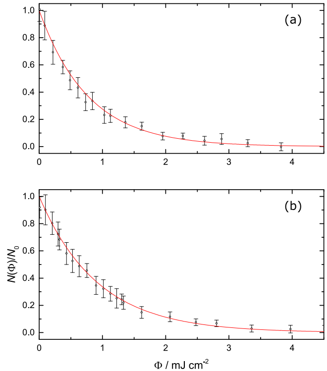
Figure 3. Photofragmentation of C_{42}H_{18}^+-He as a function of laser fluence at (a) \lambda = 8281 \text{ \AA} and (b) \lambda = 8248 \text{ \AA} . Experimental data (circles) were fit with exponential functions (lines), providing information on the photofragmentation cross section. The data were corrected for the same number of background ions appearing at m/z = 526 \text{ u/e} .
