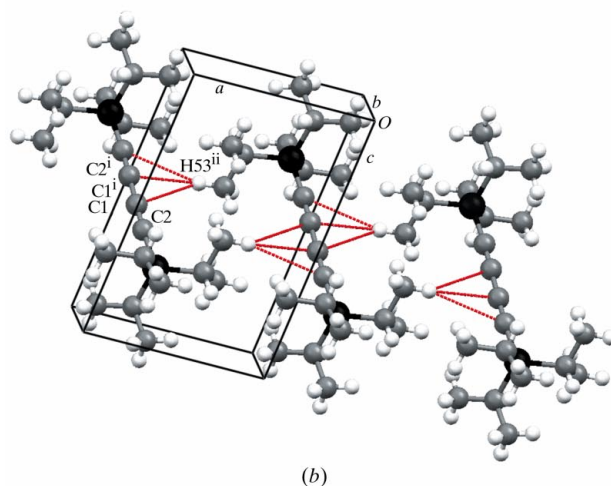
Figure 2 (a) The packing of molecules of (I), showing parts of two offset rows. (b) C-H \cdots \pi interactions between adjacent molecules in a row ( C2^i \cdots H53^{ii} = 3.2 \text{ \AA} , C1^i \cdots H53^{ii} = 2.9 \text{ \AA} and C1 \cdots H53^{ii} = 3.1 \text{ \AA} ). [Symmetry codes: (i) -x + 2, -y + 1, -z + 1 ; (ii) 1 - x, 1 - y, 1 - z .]
