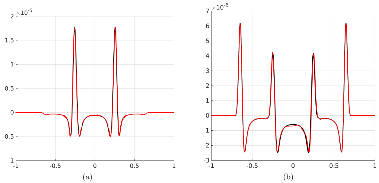
Figure 5: Periodic medium. Horizontal cross-sections (a) at x_2 = 0 in the x_1 direction and (b) at x_1 = 0 in the x_2 direction of the displacement fields u^0 (black) and u^\varepsilon (red) at the final time T = 0.2 , with \varepsilon = 1/100 .
