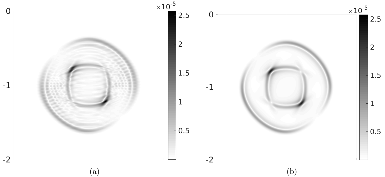
Figure 8: Horizontally layered material. Snapshots at time t = 0.1 of (a) the amplitude of the reference solution u^\varepsilon and (b) the amplitude of the homogenized solution for \varepsilon = 1/50 .
