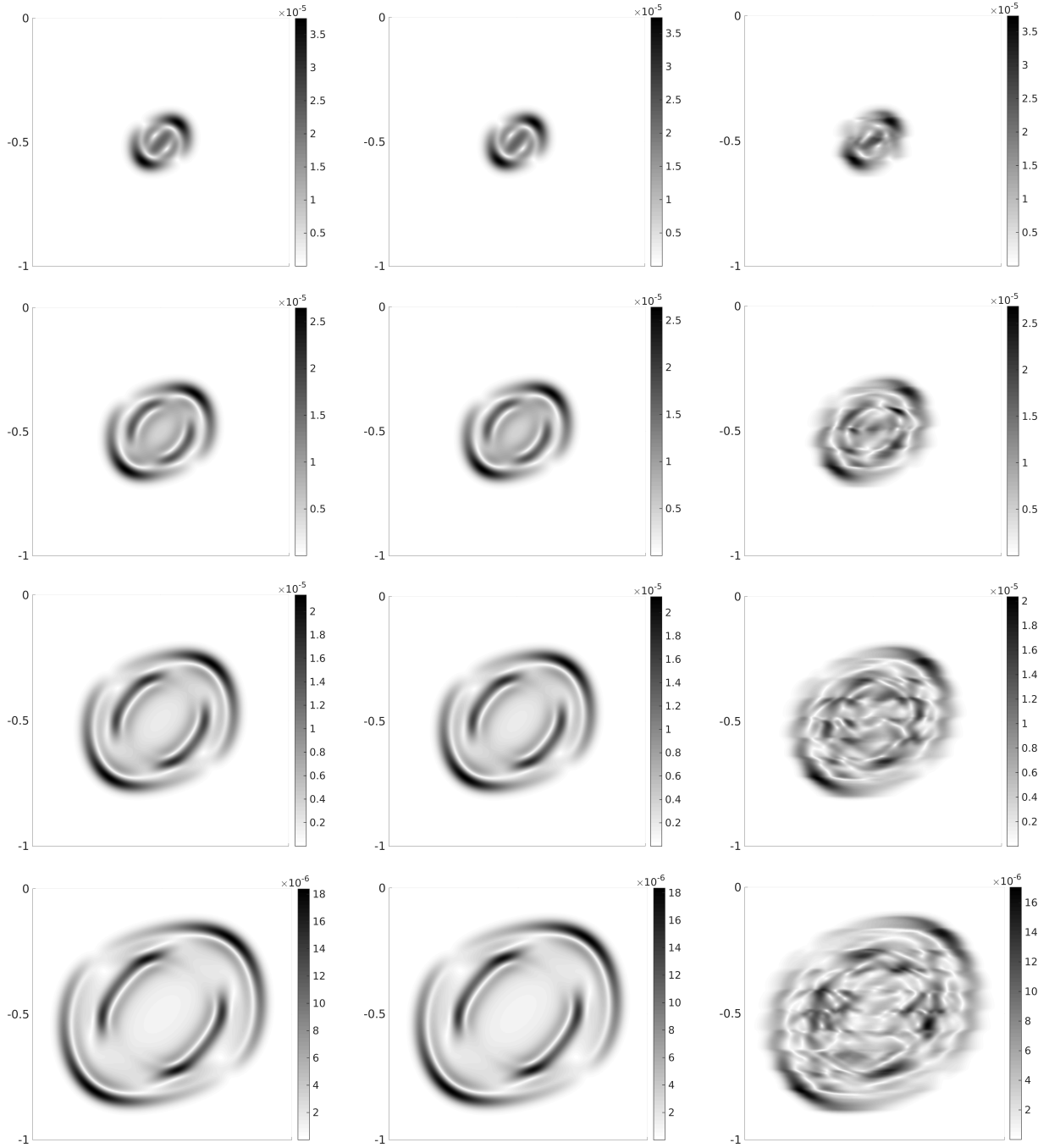
Figure 10: Layered von-Karman random medium. Snapshots at time t = 0.025, 0.05, 0.075, and 0.1 of the amplitudes of the numerical homogenized solution ( 1^{st} column), the homogeneous solution with the tensor (25) ( 2^{nd} column), and the reference heterogeneous solution u^\varepsilon ( 3^{rd} column).
