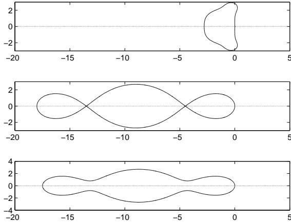
Fig. 4.1 Stability regions: fourth-order RK4 (top) and first-order 3-stage Chebyshev methods without damping (middle) and with damping (bottom). The stability regions of the RK-Chebyshev method is about nine times larger than that of the standard RK4.
