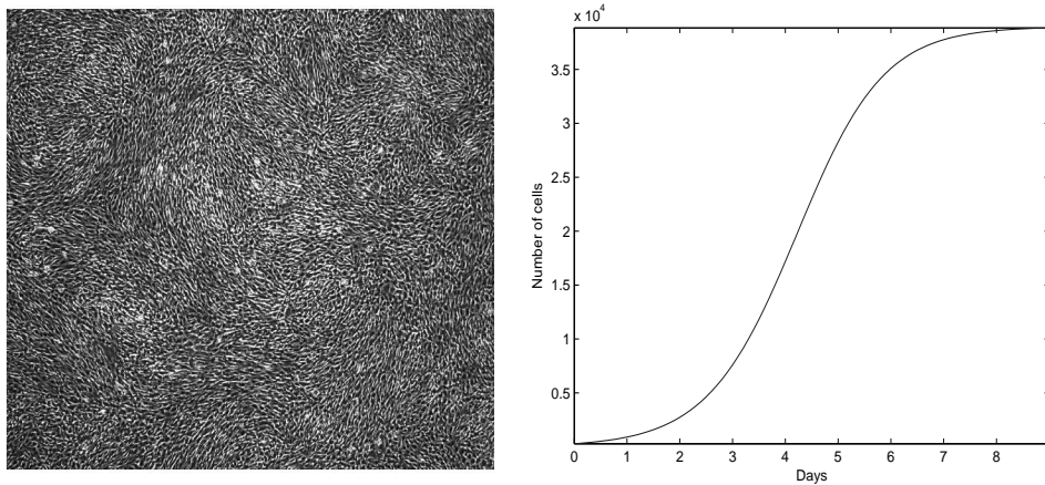
Fig. 2.1 Original image of AHAC cells cultured with TFP at day 9 near confluence (left). Sigmoidal evolution of number of cells vs. time (right)
