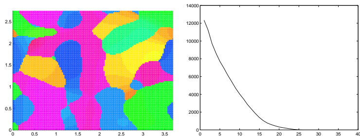
Fig. 6.3 The cell density is shown at confluence for the standard parameter values in table 6.1, but with smaller angular diffusion coefficient: \epsilon_1 = 0.0025 .
