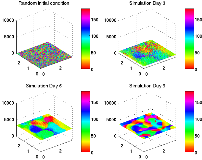
Fig. 6.1 Snapshots of the cell density at different times. At each point (x, y) in the computational domain, the marginal angular density of C is shown; the color represents the angle for which C(x, y, \theta, t) is maximal.
