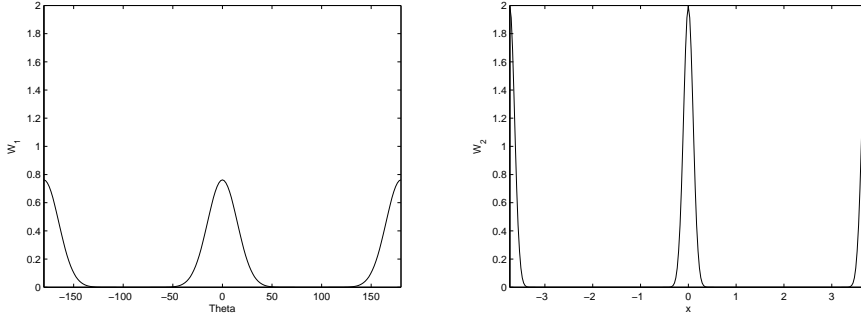
Fig. 3.1 The angular and spatial interaction kernels from (3.3), (3.4): W_1 (left) and W_2 (right).
