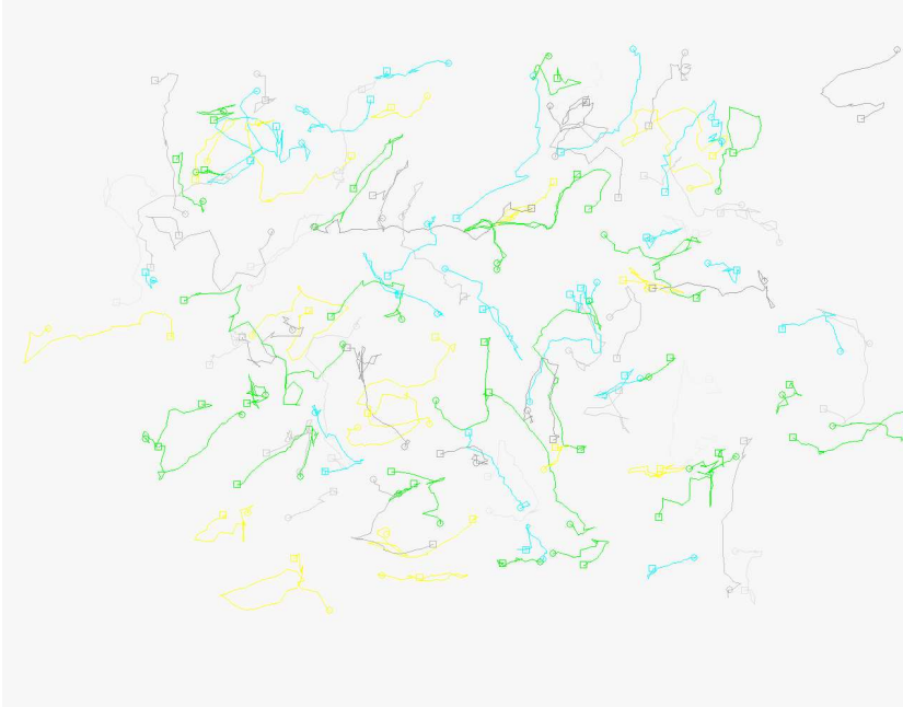
Fig. 2.2 Tracking of individual cells at density 20000/\text{cm}^2 .
