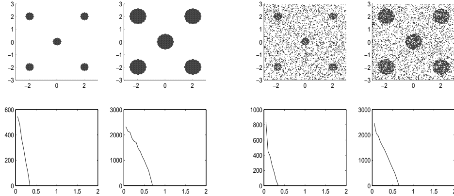
Fig. 2.5 Estimate of cluster size from synthetic texture images (top left) and corresponding cluster size function r(s) , as in (2.1) (bottom left). The intersection of r(s) with the s -axis yields a robust estimate of the cluster size, even in the presence of added random noise (right).
