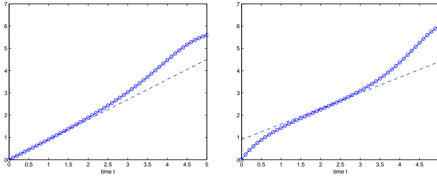
Fig. 5.1 Comparison of the growth rates for the fully nonlinear and the linearized models: Left \rho = 0 : The dashed line is \lambda t , where \lambda is given by the solution of the linear stability problem, equation (5.5). The curve with the circles denotes \ln(\|C\|) . Right \rho = 0.2 : The dashed line shows the long-time behaviour of the solution of (5.10). The curve with circles results from the solution to the full problem (3.5).
