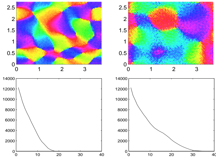
Fig. 6.4 The cell density is shown at confluence for the standard parameter values in table 6.1, but with a larger value in the critical angle: \alpha = 40^\circ (left) and \alpha = 60^\circ (right).
