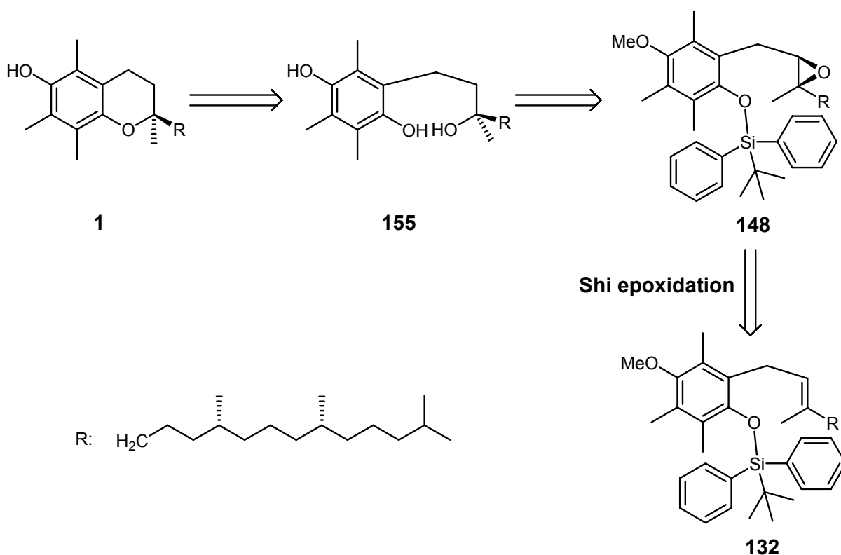
Figure 66: Retrosynthetic analysis for the transformation of 148 to 1 .
