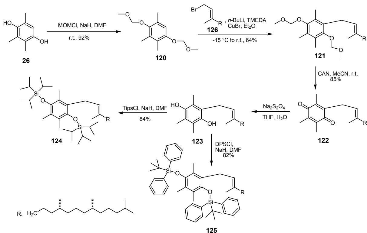
Figure 55: Synthesis of bis-protected phytyl hydroquinones 124 and 125 .
