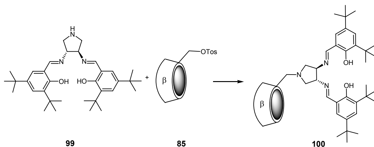
Figure 35: Attachment of salen ligand 99 to CD.
