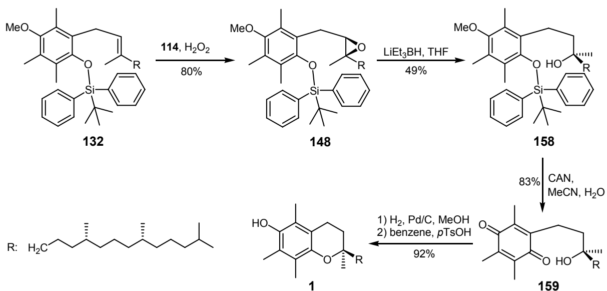
Figure 68: Alternative synthetic pathway for the transformation of olefin 132 to \alpha -tocopherol ( 1 ).
