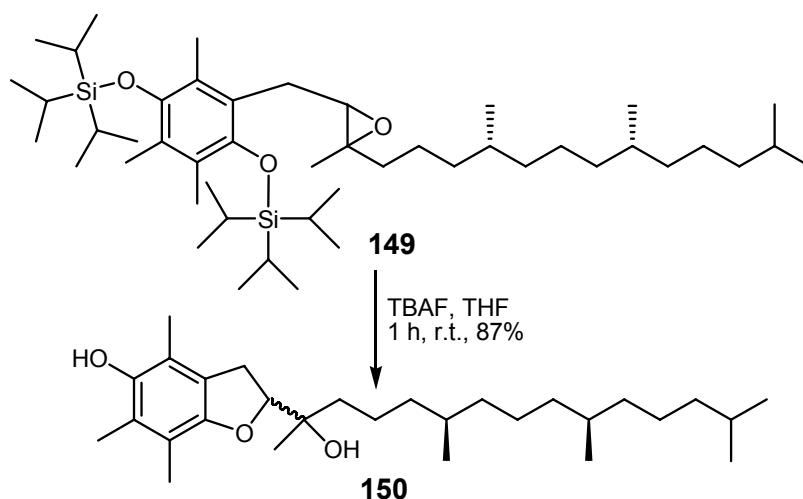
Figure 62: Cleavage of the TIPS ether, yielding 5-membered ring product 150 .
