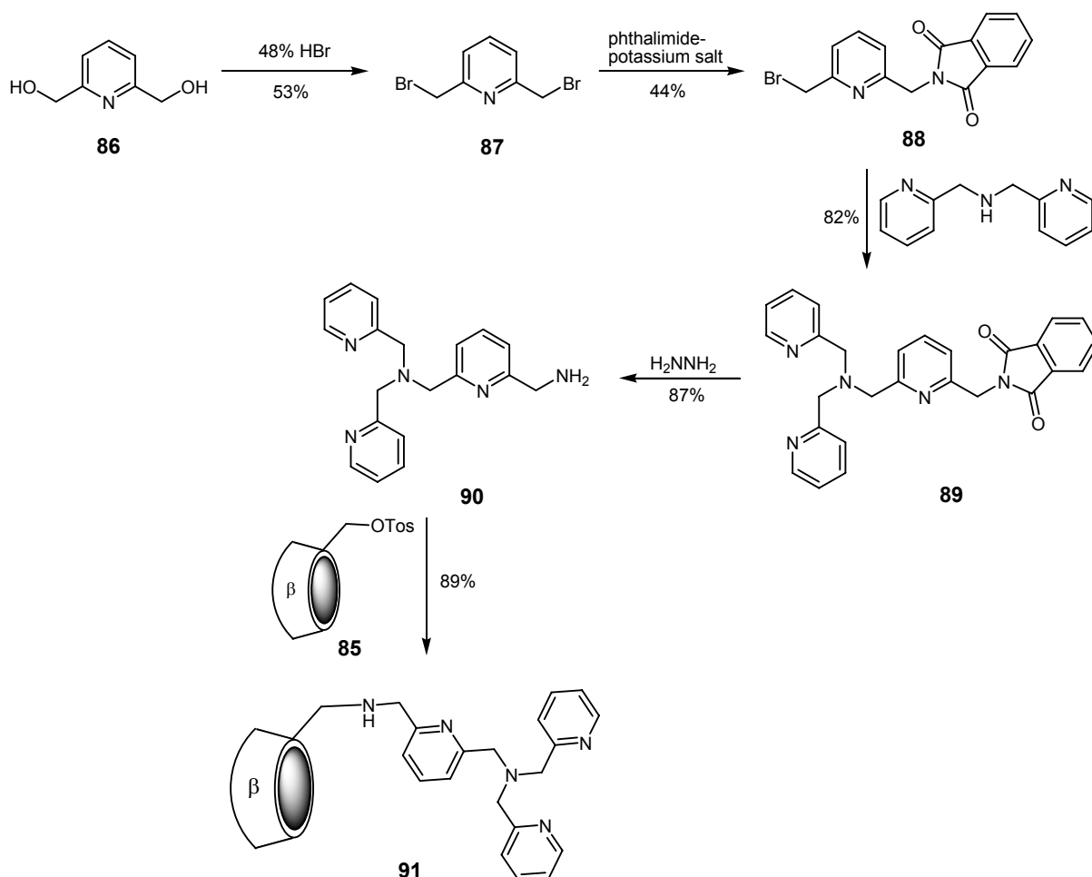
Figure 29: Synthesis of CD-ligand 91 .
