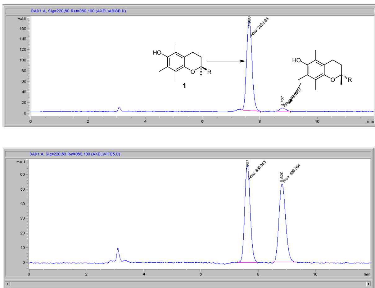
Figure 69: Top: HPLC chromatogram of the products of the cyclisation of 157 . Bottom: HPLC chromatogram of commercial all racemic \alpha -tocopherol.
