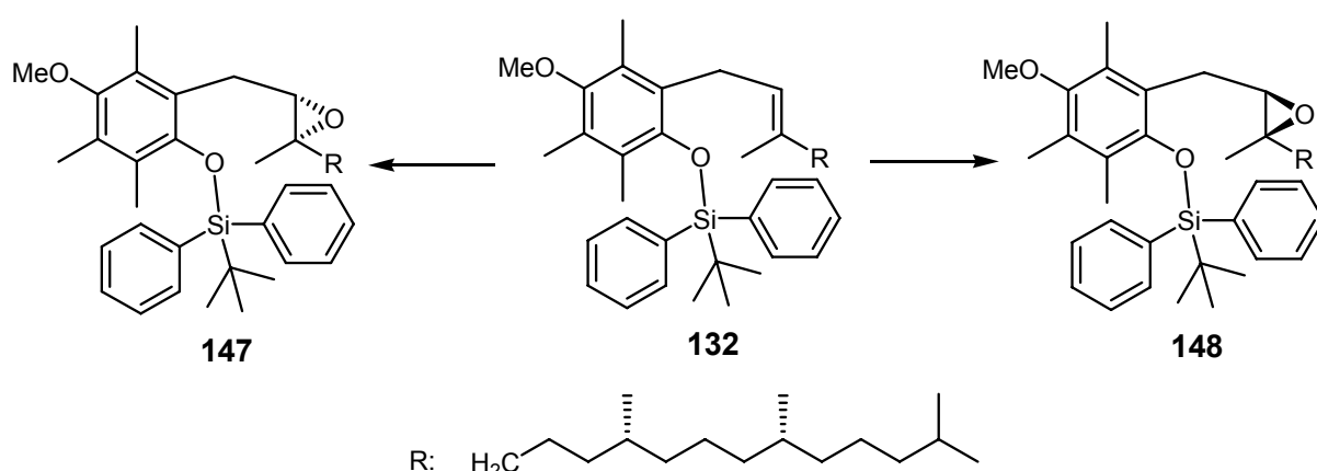
Figure 70: Asymmetric epoxidation of 132 giving 147 or 148 .
